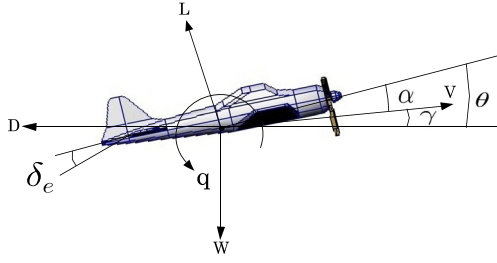
Fig. 1 Pure pitching motion
