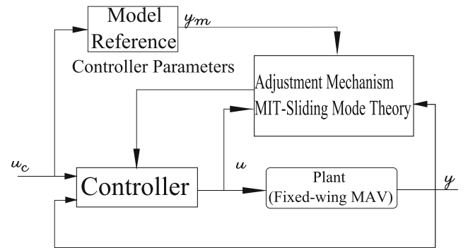
Fig. 5 Block diagram of the MRAS
