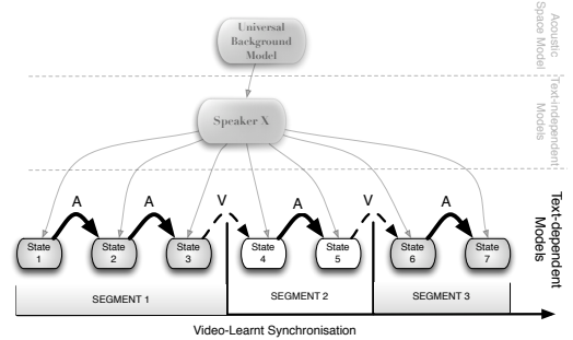
Fig. 2. Use of an Video-Learnt Segmentation in the bottom layer of the EBD system to constrain the Viterbi decoding and reinforce the TSI in the utterance SCHMMs. The V labelled transitions are constrained by the video-learned segmentation as the A labelled ones still unchanged
