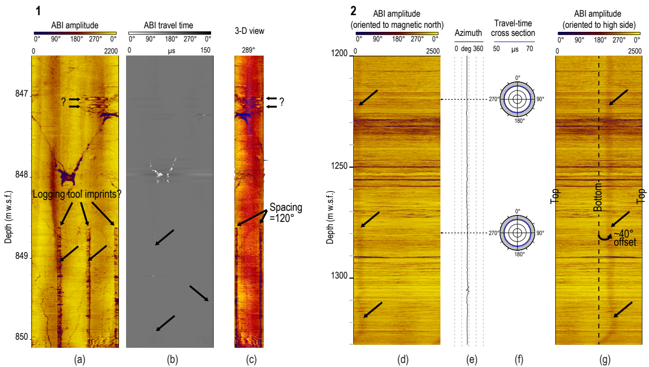
Figure 8. Marks on the borehole wall. (1) possible tool imprint oriented to 120°, and residue possibly left in mud residue by arms of the mechanical caliper. (2) ABI image oriented with respect to the magnetic north (d) and to the high side, (g) illustrating that the continuous regular narrow dark stripe (black arrows) is closely related to borehole inclination and may be the result of the drill pipe rubbing on the borehole wall. (f) travel-time cross section (magnetic north orientation) illustrates a regular borehole shape with no evidence for groove cut to be associated with the narrow dark stripe. Note that the travel-time cross sections' lower limit has been set to 50 μs.
