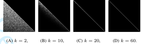
Fig. 2 The convergence procedure of D_k in CSVD-QR.
