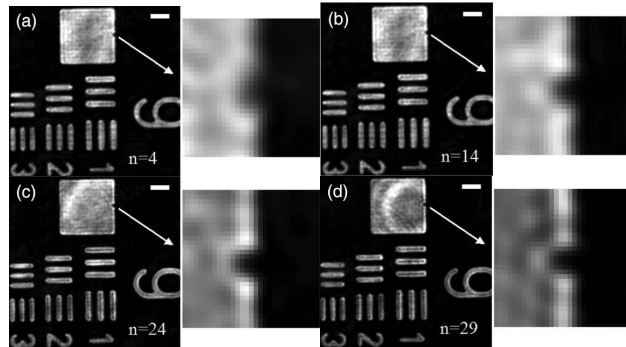
Fig. 3. Reconstruction of high NA holograms for various defocus. (a) z' - z_{p'} = -47.69 \mu\text{m} . (b) z' - z_{p'} = -23.39 \mu\text{m} . (c) z' - z_{p'} = 0.8 \mu\text{m} . (d) z' - z_{p'} = 12.84 \mu\text{m} . Scale bar is 3 \mu\text{m} .
