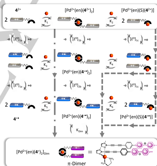
Figure 6. Schematic representation of the chemical and electrochemical reactions and equilibria involving 4 2+ and of cis -[Pd(NO 3 ) 2 (en)]. Each Electrochemical steps (E) represented in this mechanism are mono-electronic
