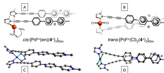
Figure 10. 2D representations (A,B) and optimized structures (C,D) of cis -[Pd 2+ (en)(4 + ) 2 ] Dim and trans -[Pd(Cl) 2 (4 + ) 2 ] Dim calculated at the BP86/6-31G*+LANL2DZ level of theory.
