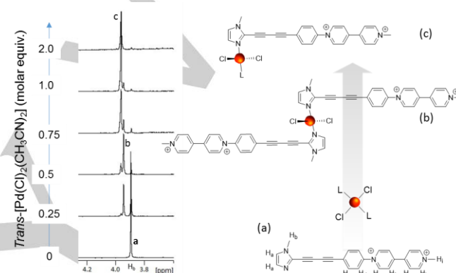
Figure 4. Partial ^1\text{H} NMR spectra of \mathbf{4}(\text{PF}_6)_2 (2 mM, \text{DMF-}d_7 , 500 MHz) recorded during the addition of trans - [\text{Pd}(\text{Cl})_2(\text{CH}_3\text{CN})_2] (number of equivalents, n_{\text{eq}} Pd, written on the left). The signal corresponding to the imidazole moieties of \mathbf{4}^{2+} and trans - [\text{Pd}(\text{Cl})_2(\mathbf{4}^{2+})_2] trans - [\text{Pd}(\text{Cl})_2(\text{L})(\mathbf{4}^{2+})] are labelled with a, b, and c respectively.
