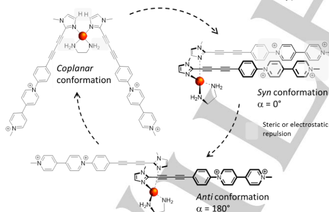
Figure 3. Representation of the syn , anti and coplanar conformations of cis - [\text{Pd}^{2+}(\text{en})(\mathbf{4}^{2+})_2]
