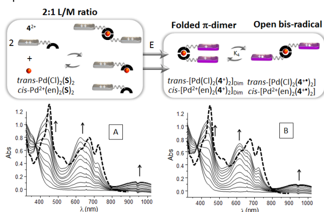
Figure 9. Superposition of UV/Vis absorption spectrum of 4^{2+} (dashed line) and spectra recorded during the exhaustive reduction (one electron per viologen) of 4^{2+} in presence of 0.5 molar equivalent of A) cis -[Pd(NO 3 ) 2 (en)] (full line) and B) trans -[Pd(Cl) 2 (CH 3 CN) 2 ] (full line) (DMF + 0.1 M TBAP, 0.4 mM, 15 mL, E_{\text{app}} = -0.8 V, l = 1 mm, t \approx 30 min, working electrode = Pt).
