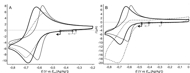
Figure 5. Raw voltametric curves measured for 4(\text{PF}_6)_2 at 0.4 mM in DMF + TBAP 0.1 M (VC, \varnothing = 3 mm, E (V) vs \text{Ag}/\text{Ag}^+ 10^{-2} M, \nu = 0.1 V s -1 ) before addition of Pd(II) (bold solid line), and after addition of 0.5 molar equivalent (thin solid line) of A) cis -[Pd(NO 3 ) 2 (en)] and B) trans -[Pd(Cl) 2 (CH 3 CN) 2 ], and after addition of A) 3 molar equivalents of cis -[Pd(NO 3 ) 2 (en)] and B) 2 molar equivalents of trans -[Pd(Cl) 2 (CH 3 CN) 2 ] (dashed line).
