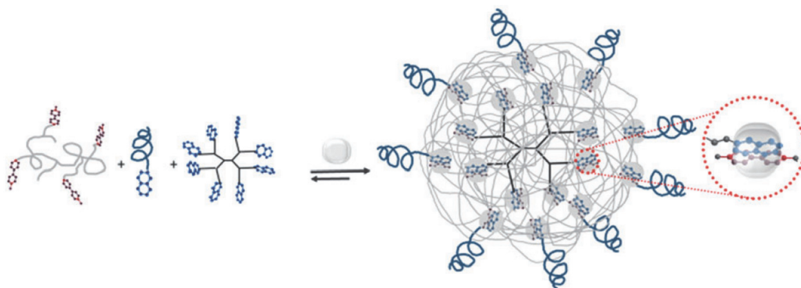
Figure 20: SNP formation starting from a first generation dendrimer (PAMAM) and other polymers. 106
