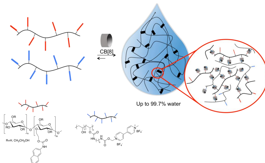
Figure 14 : Schematic representation of the 1:1:1 (CB[8]/viologen/naphthoxy) supramolecular ternary complexes yielding ultra-high water content hydrogels. 95
