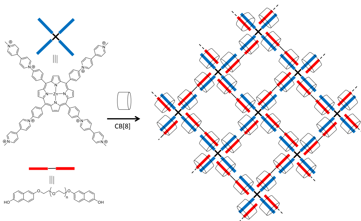
Figure 5. Schematic representation of a 2D supramolecularly polymeric pattern obtained from porphyrin-based AAAA and hydroxy naphthalene-based DD monomers. 58
