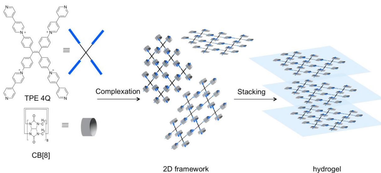
Figure 17. Hydrogel formation based on supramolecular assembly as 2D layers of a tetratopic guest and CB[8] followed by further inter layer stacking. 101
