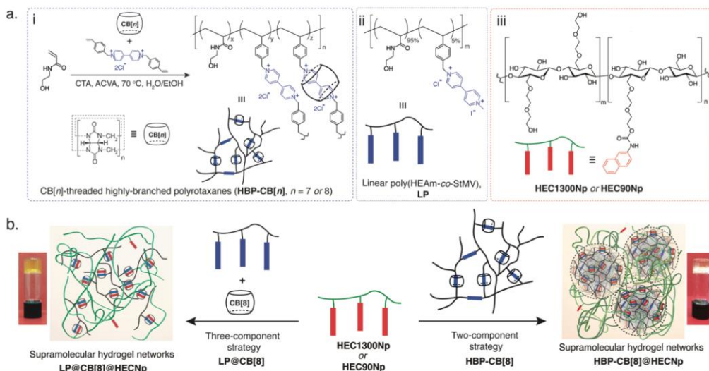
Figure 16 : a) Schematic illustration of i) synthesis of the highly branched CB[n] -threaded polyrotaxane (HBP- CB[n] ) via a semi-batch RAFT polymerization in the presence of CB[n] , ii) chemical structures of its linear analog (LP), and iii) naphthyl-functionalized hydroxyethyl cellulose (HECNp). b) Formation of hydrogel networks through a two-component strategy from HBP- CB[8] polyrotaxane (HBP- CB[8] @HECNp) or a three-component strategy from its linear analog (LP@ CB[8] @HECNp). Inset: inverted vial tests for the hydrogel networks from. 99 Reproduced from Ref. 99 with permission from John Wiley and Sons.
