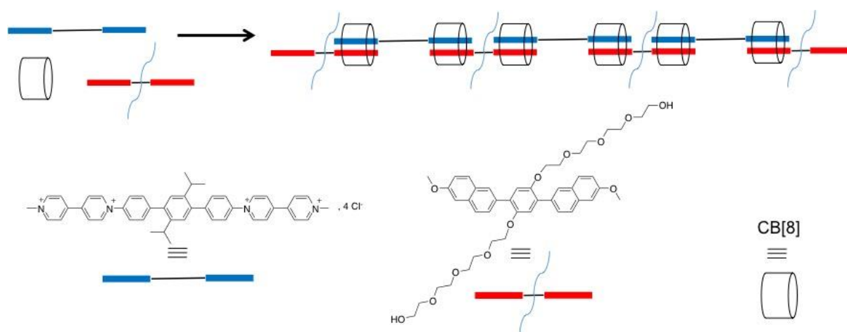
Figure 4: Supramolecular « bottlebrush » polymer constructed from rigid AA and DD type monomers. 57
