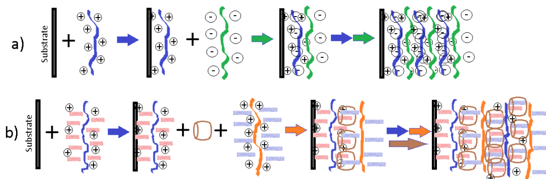
Figure 18 : Schemarepresentation of the LBL deposition technique for a): classical ion-pair formation, and b): Host-stabilized charge-transfer pair (HSCT) LBL. 104
