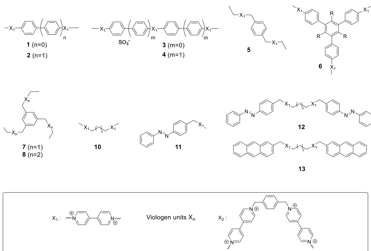
Figure 6. Viologen-based building blocks used for the construction of stimuli-responsive supramolecular polymers.
