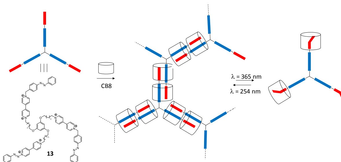
Figure 10. Schematic representation of the self-assembly process proposed with the star-shaped monomer 13 with CB[8]. 78
