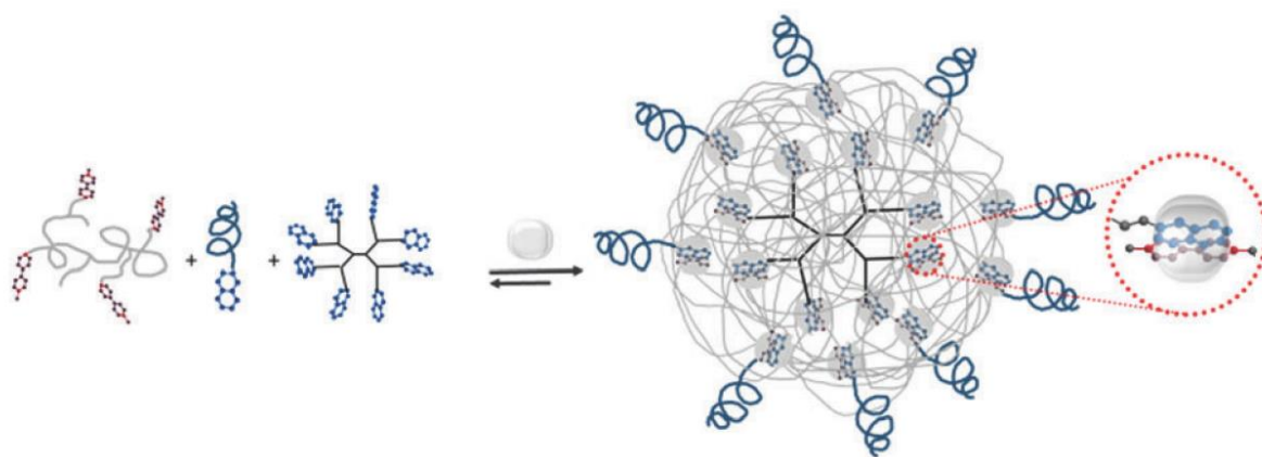
Figure 21: SNP formation starting from a first generation dendrimer (PAMAM) and other polymers. 111 Reproduced by permission of The Royal Society of Chemistry.
