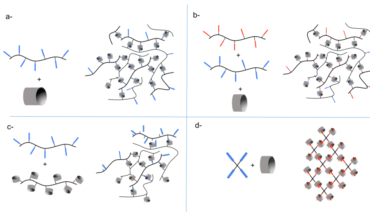
Figure 13: Four different patterns involved in the hydrogelation of CB[8]/viologen-based supramolecular assemblies.
