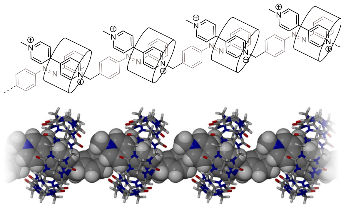
Figure 9. Schematic representation and side view of the X-ray structure of the linear supramolecular assembly obtained from 11 (Z isomer) and CB8. 76 Reproduced from Ref. 76 with permission from the American Chemical Society.
