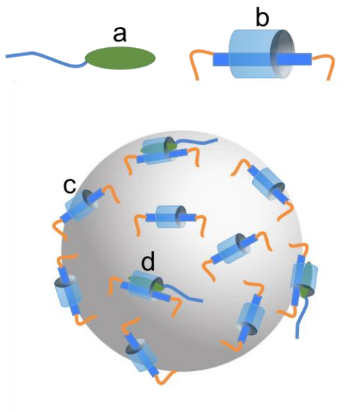
Figure 22: The catenane immobilization strategy over a spherical particle, a) an electron donor, b) a CB[8] pseudorotaxane containing a viologen core, c) the pseudorotaxane is immobilized, d) the pseudorotaxane accommodates the electron donor, forming a host-stabilized ternary charge-transfer complex. 120
