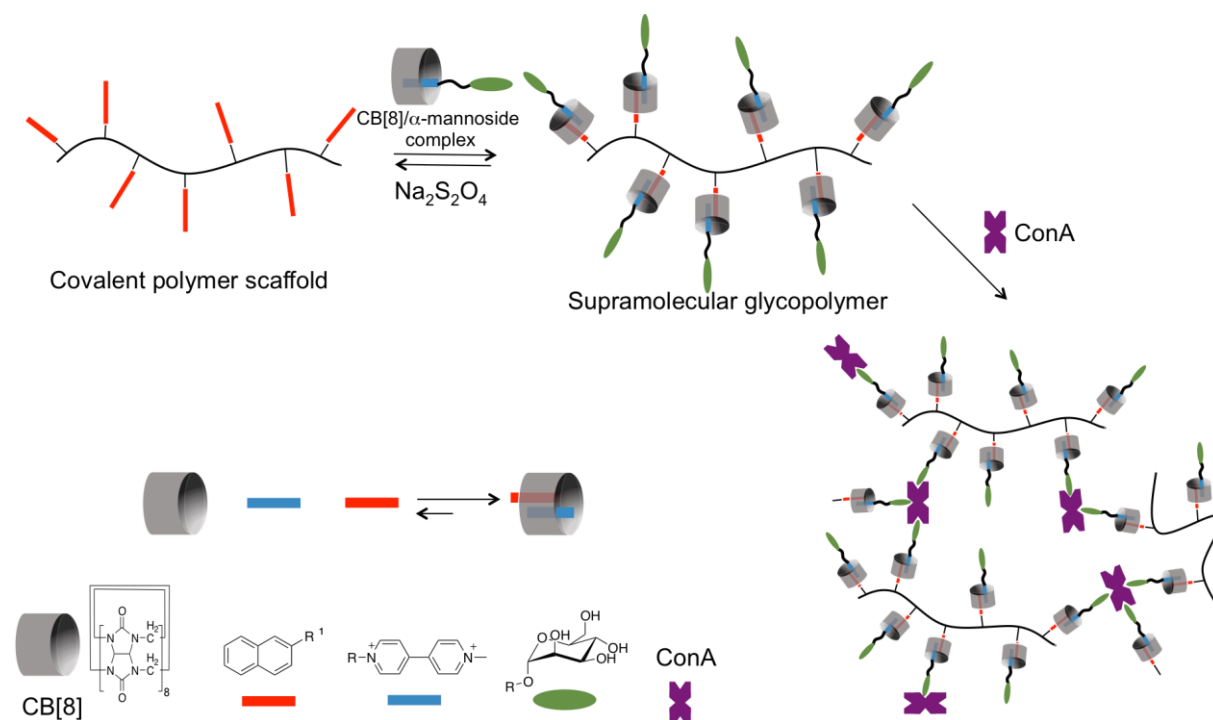
Figure 11. a) Reversible Formation of aviologene/CB[8]- glycopolymer conjugate and b) self-assembly of the glycopolymer with a manose-specific lectin (concanavalin A). 79
