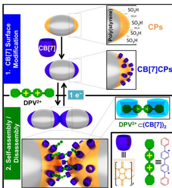
Figure 19: Self aggregation of polymeric colloidal particles using 2 hosts ternary cavipect and diphenylviologen (DPV). 105, 106 Reproduced from Ref. 106 with permission from The American Chemical Society.
