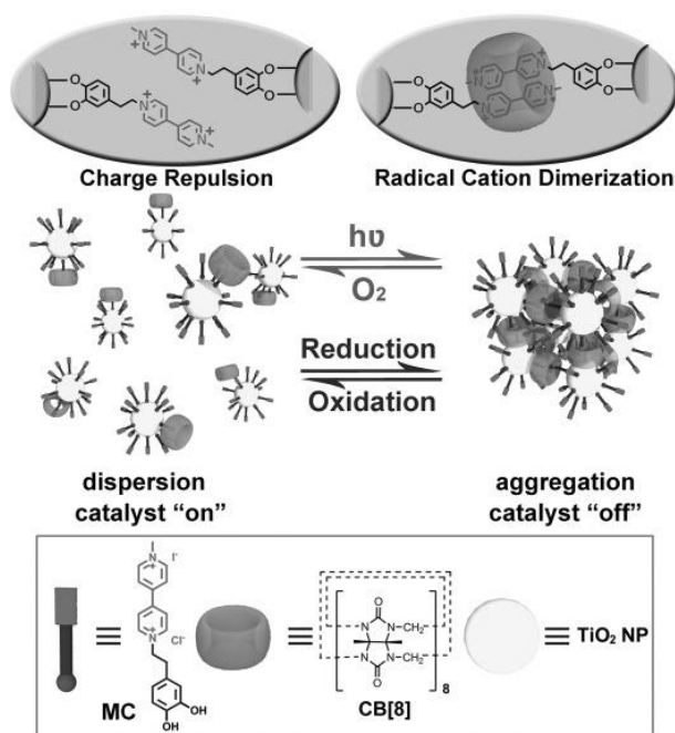
Figure 20: Reversible self-assembly of \text{TiO}_2 nanoparticles modified with methyl viologens and cucurbit[8]uril. Aggregation may be triggered by light, or chemical reduction to form radical cations. Reoxidation of the later causes disassembly. 109 Reproduced from Ref. 109 with permission from John Wiley and Sons.
