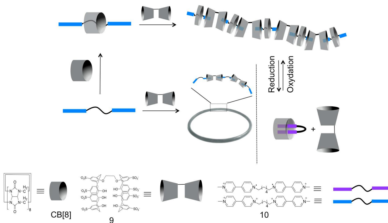
Figure 8. Schematic representation of the CB[8]-based self-assembly and of the effect of redox stimulation. 75
