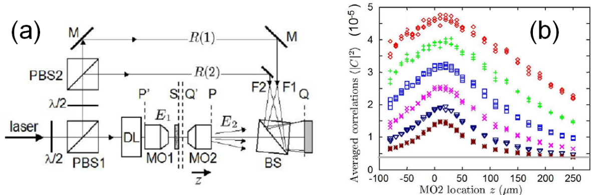
Fig.1 (a) Holographic experimental setup. (b) Residual correlation of the transmitted field. The horizontal axis is SQ' . The sample transverse size is L=70 \mu\text{m} red, 50 \mu\text{m} green, 35 \mu\text{m} blue.... The horizontal grey line is the residual correlation expected for N_1=N_2 .
