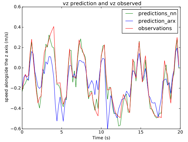
Figure 2. comparison of ARX and neural network model on non linear dynamic.
