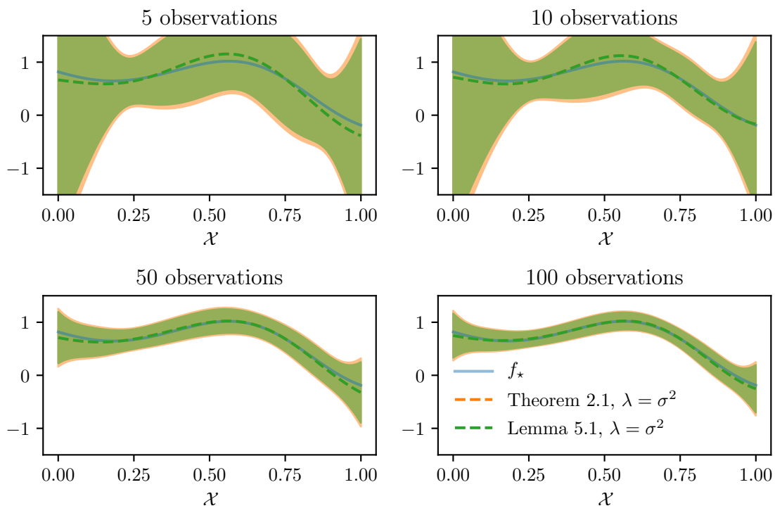
Figure 2: Confidence interval of Theorem 2.1 and Lemma 5.1 (Wang and de Freitas, 2014).
