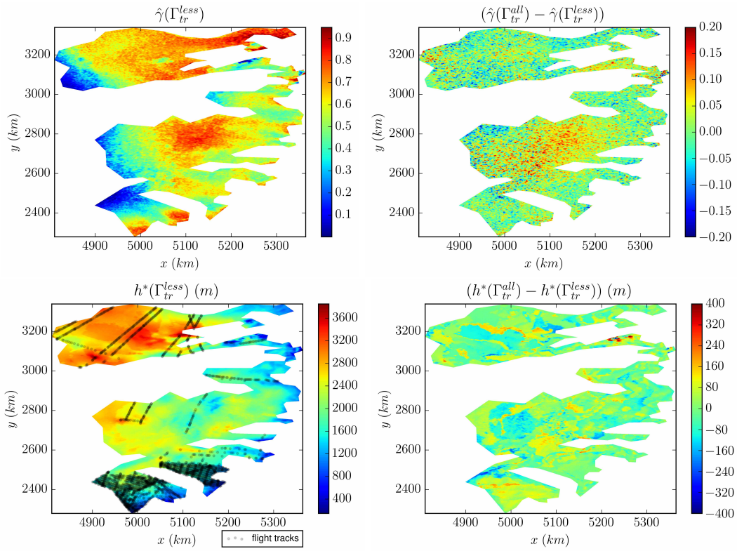
Figure 10. Domain \Omega_p=\text{Ant3} : comparison if not considering the flights tracks indicated in Fig.9 (Up)(L). (Up)(L) Field \hat{\gamma}(\Gamma_{tr}^{less}) (i.e. without the flights tracks indicated in Fig.9 (Up)(L)). (R) Difference (\hat{\gamma}(\Gamma_{tr}^{all}) - \hat{\gamma}(\Gamma_{tr}^{less})) . (Down)(L) Inferred thickness h^*(\Gamma_{tr}^{less}) . (R) Difference between the two estimations: (h^*(\Gamma_{tr}^{all}) - h^*(\Gamma_{tr}^{less})) .
