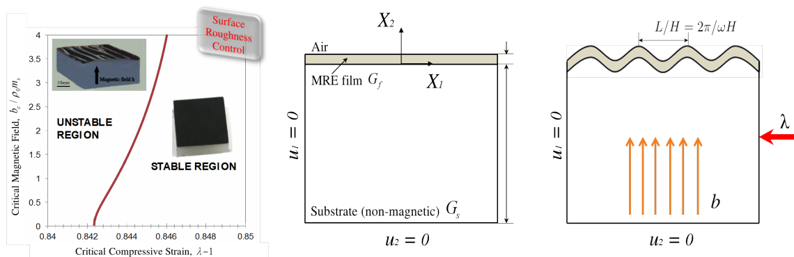
FIGURE 1 – (a) Qualitative stability phase diagram of the MRE film-substrate block ; (b) Pre and post-bifurcation regime of the block after the application of magneto-mechanical loadings
