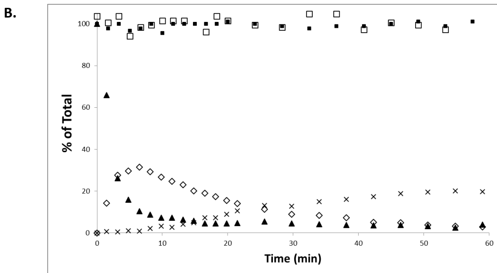
Figure 3. Drug release in reductive conditions (3 equiv. sodium dithionite, \text{CH}_3\text{CN}/0.1 \text{ M} cacodylate buffer, pH 7.4, 37^\circ\text{C} ) and stability in plasma assessed by NMR ^{31}\text{P} : A. Stacked NMR ^{31}\text{P} spectra; a. prodrug 31f , 17.99 ppm; b. phosphoramidate anion, 12.39 ppm (proven by MS-HPLC, data not shown); c. inorganic phosphate, 0 ppm. Other signals are relatives to solvolysis, buffer and reductive adducts or transient unknown by-products. Chemical shifts are reported relative to the \text{Ph}_3\text{PO} reference. B. Representative time course of phosphoramidate 31f cleavage (▲), substituted bis(2-chloroethyl)phosphoramidate anion formation (◇) and inorganic phosphate formation (×) upon incubation of the prodrug with sodium dithionite in cacodylate buffer; Stability of phosphoramidate 31f in cacodylate buffer (■) and in rabbit plasma (□). Data points were measured from NMR ^{31}\text{P} areas (average of two runs).
