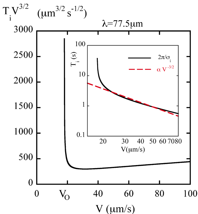
FIG. 11: Evolution with the pushing velocity V of the period T_i = 2\pi/|\sigma_i| of the 2\lambda -O mode at \lambda = 77.5\mu\text{m} , following the imaginary part of the eigenvalue \sigma_i provided by the system (27) (28). To compare with the experimental and numerical trend (11), the period T_i is multiplied by V^{3/2} . The nearly constant value reached shortly after the occurrence of oscillations at V_O = 18\mu\text{m}\cdot\text{s}^{-1} agrees with the observed relationship (11). The insert shows data in log-log coordinates and a comparison with the trend T_i \propto V^{-3/2} of relation (11).
