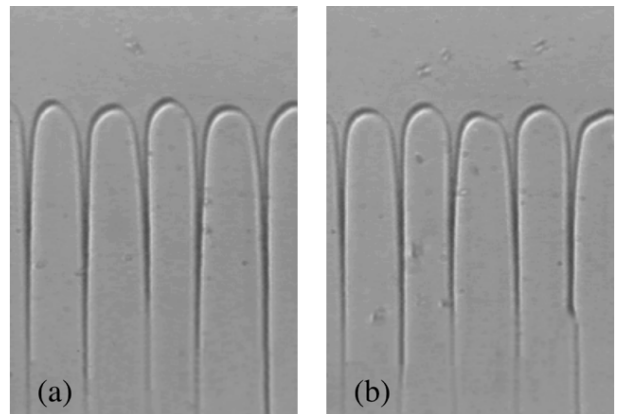
FIG. 13: Cell oscillations from tip to tail. Same parameters as in figure 12. Snapshots (a) and (b) are distant from a half-period T/2 = T_f = 141\text{s} . On each of them, cell widths are nearly the same at cell tips but significantly different at cell tails. On each cell, the modulations of cell width from tip to tail thus encode the oscillation of cell tip over a long time, here about T/3 , before the grooves end. The mean cell spacing is 110\mu\text{m} .
