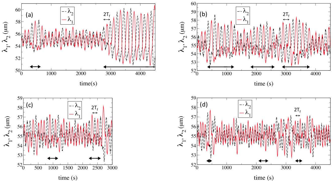
FIG. 14: (Color online) Numerical simulations of parametric excitations with a forcing amplitude V_1 = 0.2\mu\text{m}\cdot\text{s}^{-1} . The basic state refers to V_0 = 7\mu\text{m}\cdot\text{s}^{-1} , \lambda = 65\mu\text{m} , and the forcing period T_f is (a) 115 s, (b) 110 s, (c) 90 s, (d) 80 s. The variables \lambda_i refer to cell width of neighbor cells. Double arrows indicate oscillations at the double period 2T_f , with a phase opposition between neighbor cells. They correspond to a parametrically forced 2\lambda -O mode. Figure (a) shows the growth and saturation of a robust parametrically excited mode involving, as the 2\lambda -O mode, a period 2T_f for both \lambda_i and phase opposition between them. The remaining figures show that the parametric mode appears more and more intermittently as T_f decreases below its value in (a).
