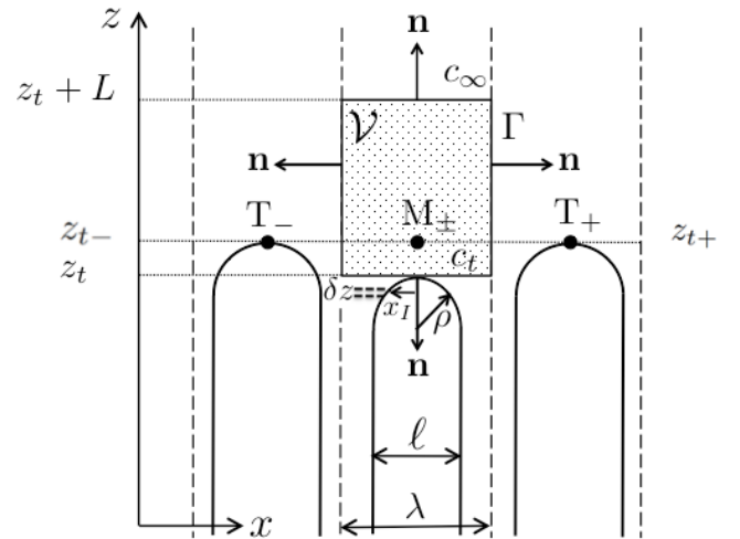
FIG. 9: Sketch of the domain used for modeling. Cells geometries are taken as circular tips of radius \rho = \ell/2 followed by a constant width \ell . The coordinates of a cell interface point are (x_I, z_I) . The tips of the first neighbor cells are designed by T_- and T_+ . The points in the middle of the central cell that stand at the same height as the neighbor cell tips are called M_\pm . A control volume \mathcal{V} of width \lambda and height L > l_D is defined in which solute evolution is determined from the solute fluxes across its sides. In addition to the usual advection and diffusion fluxes, transversal fluxes are induced here by the shift of tip position between a cell and its neighbors. The contour of the box is labelled \Gamma and its outward normals \mathbf{n} . At a finer scale, the evolution of solute concentration in elementary bands \delta z around the cell tip enables the implication of transversal fluxes on the evolution of tip curvature radius \rho to be determined.
