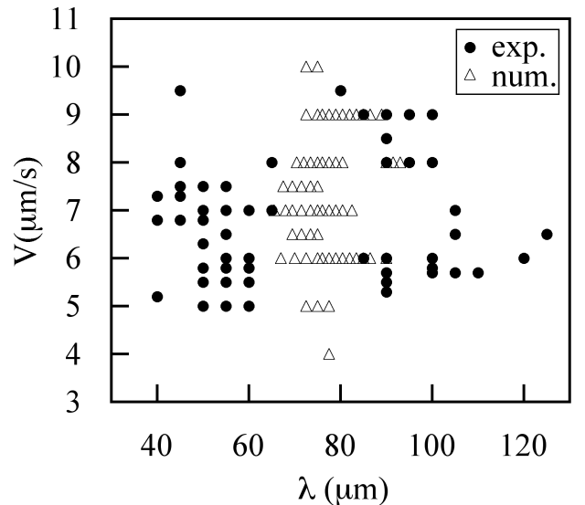
FIG. 4: Existence diagram of the 2\lambda -O mode obtained at G = 110\text{K}/\text{cm} : different symbols correspond to the occurrences found experimentally (full circles) and numerically (empty triangles).
