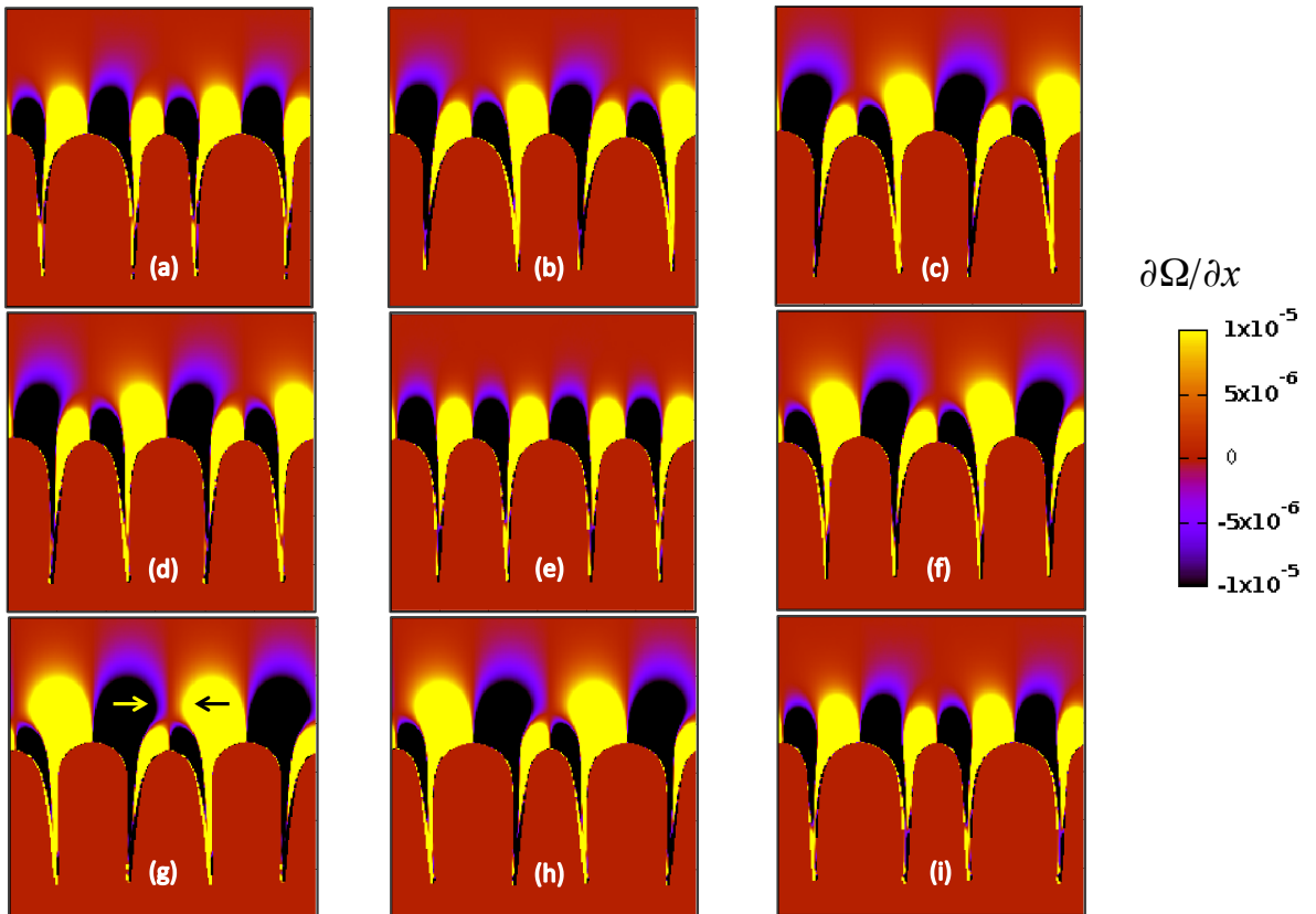
FIG. 8: (Color online) Time evolution of the field \partial\Omega/\partial x for the same parameters as those of Fig. 7. The two arrows in panel g indicate the orientations of the horizontal solute currents, proportional to -\partial\Omega/\partial x , that converge toward the central cell. At the bottom and the top of the frames, the zero current areas respectively represent the solid and the far-field liquid.
