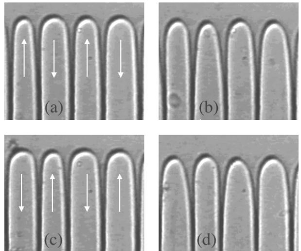
FIG. 12: Experimental evidence of a parametrically excited 2\lambda -O mode over a cycle. G = 140\text{K/cm} , V_0 = 7\mu\text{m/s} , V_1 = 0.5\mu\text{m/s} and T_f = 141\text{s} . The snapshots show cell oscillations in the vicinity of cell tips over an oscillation period T = 282\text{s} that is twice the forcing period T_f . The delay between them is a quarter of period. Arrows denote the direction of cell velocities and the mean cell spacing is 85\mu\text{m} . Each snapshot shows phase opposition between neighbor cells. These features correspond to those a 2\lambda -O mode parametrically excited at a forcing period T/2 .
