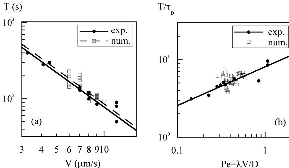
FIG. 5: Log-log plot of (a) the oscillation period T vs pushing velocity V and (b) T/\tau_D vs Pe . Full circles for experimental data, empty squares for numerical data. Data are fitted with respect to relation (11) in (a) and to relation (12) in (b). Continuous or dotted line for a fit to experimental or numerical data.
