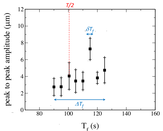
FIG. 15: Peak to peak amplitude of the driven 2\lambda -O mode as a function of the driving period T_f . Average velocity V_0 = 7\mu\text{m}/\text{s} , velocity amplitude V_1 = 0.2\mu\text{m}/\text{s} , spacing 2\lambda = 130\mu\text{m} . Amplitude is maximum for T_f = 115\text{s} close to T/2 = 100.5\text{s} . The shift (T_f - T/2) refers to damping and anharmonicity of the oscillator.
