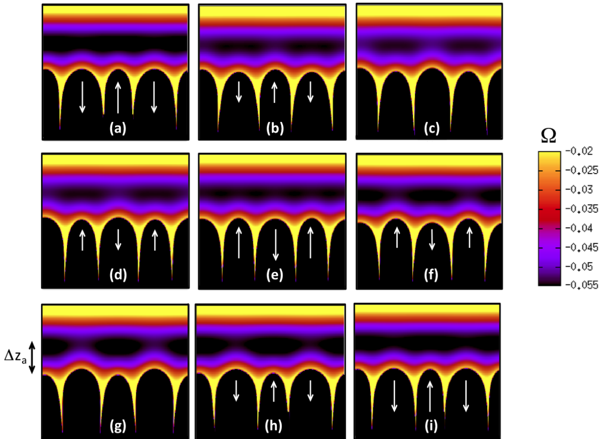
FIG. 7: (Color online) Time evolution of the 2\lambda -O mode obtained numerically. The pushing velocity is V = 9\mu\text{m/s} and the image width is 310\mu\text{m} . Solid cells appear in black in the lower part of the panels and white arrows indicate the cell tip velocities. In the liquid phase above them, isosurfaces are drawn for the constitutional undercooling \Omega defined in the text. A complete oscillation period, T \simeq 108\text{s} is swept, the frames respectively corresponding to times (a) 0; (b) T/8 ; (c) T/4 ; (d) 3T/8 ; (e) T/2 ; (f) 5T/8 ; (g) 3T/4 ; (h) 7T/8 ; (i) T .
