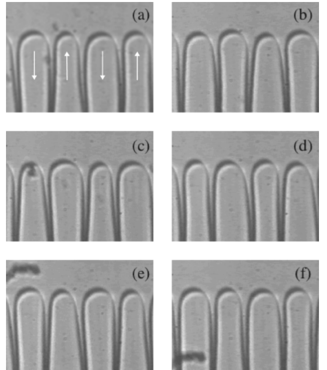
FIG. 1: Experimental evidence of a 2\lambda -O mode. From (a) to (f), six successive snapshots of the same front are shown at time intervals of 20s over a cycle. The pushing velocity is V = 8 \mu\text{m/s} , the image width is 280 \mu\text{m} , the oscillation period 100s and the thermal gradient G = 110\text{K/cm} . Snapshots (a) and (f) thus refer to the same phase of the cycle. Oscillations of tip position are tiny but those of cell width and of tip curvature are noticeable. First neighbor cells are in phase opposition and arrows in snapshot (a) indicate the direction of cell velocities in the frame of the thermal gradient.
