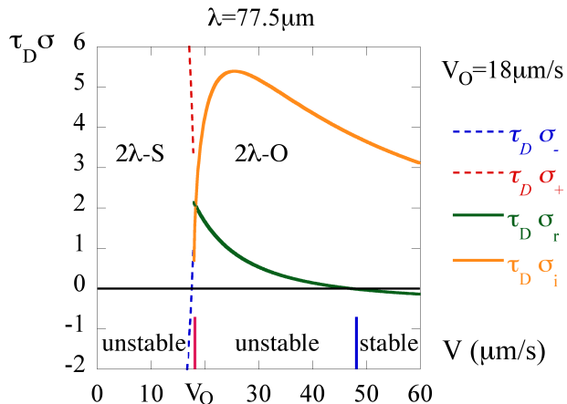
FIG. 10: (Color online) Evolution of the eigenvalue spectrum with V for modulations at two cell spacings. Dashed lines : real eigenvalues \sigma_{\pm} with \sigma_{-} < \sigma_{+} ; full lines : complex eigenvalues with \sigma_r and \sigma_i the real and imaginary parts. As V increases, a transition from 2\lambda -S to 2\lambda -O instability is encountered at V_O = 18 \mu\text{m}\cdot\text{s}^{-1} . At larger velocity, the 2\lambda -O instability restabilizes as the real part \sigma_r turns negative.
