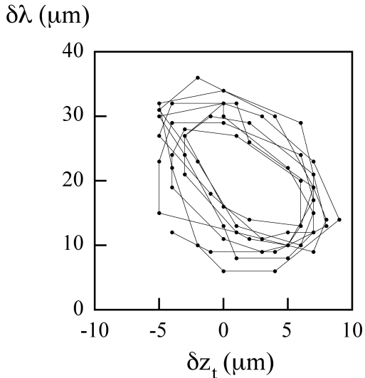
FIG. 2: Limit cycle of oscillating cells obtained from the differences of cell tip positions \delta z_t and cell widths \delta\lambda between two neighbor cells. V = 13\mu\text{m}\cdot\text{s}^{-1} , \lambda = 45\mu\text{m} , G = 140\text{K}/\text{cm} .
