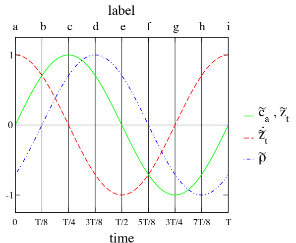
FIG. 6: (Color online) Time evolution of the fluctuations (denoted by a tilde) of four different parameters (schematic representation). The fluctuations of a given parameter are defined as its instant value minus its average value and they are normalized to one here. The parameters represented are the solute concentration at a fixed distance above the cell tip, \tilde{c}_a , and three geometric parameters of the cell tip: position \tilde{z}_t , velocity \dot{\tilde{z}}_t , and radius of curvature \tilde{\rho} . The oscillation time period is denoted by T and labels a to i refer to those used in Figs. 7 and 8
