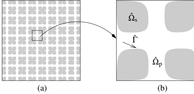
Figure 1: Periodic porous medium : (a) Macroscopic sample ; (b) Periodic cell \hat{\Omega} .
