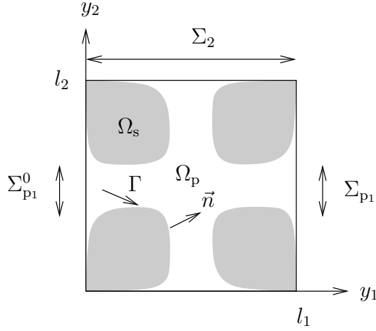
Figure 2: Two-dimensional periodic cell \Omega .
