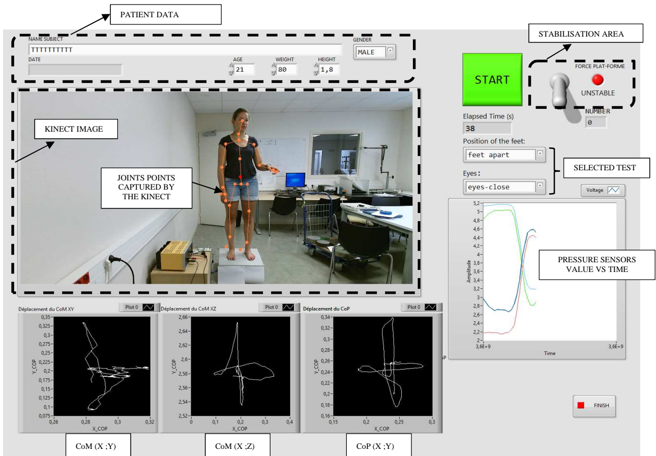
Fig 2. Human Computer Interface (HCI) designed with therapists.
