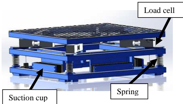
Fig 1: CAD model of the experimental platform developed in GI-Nova Centre.
