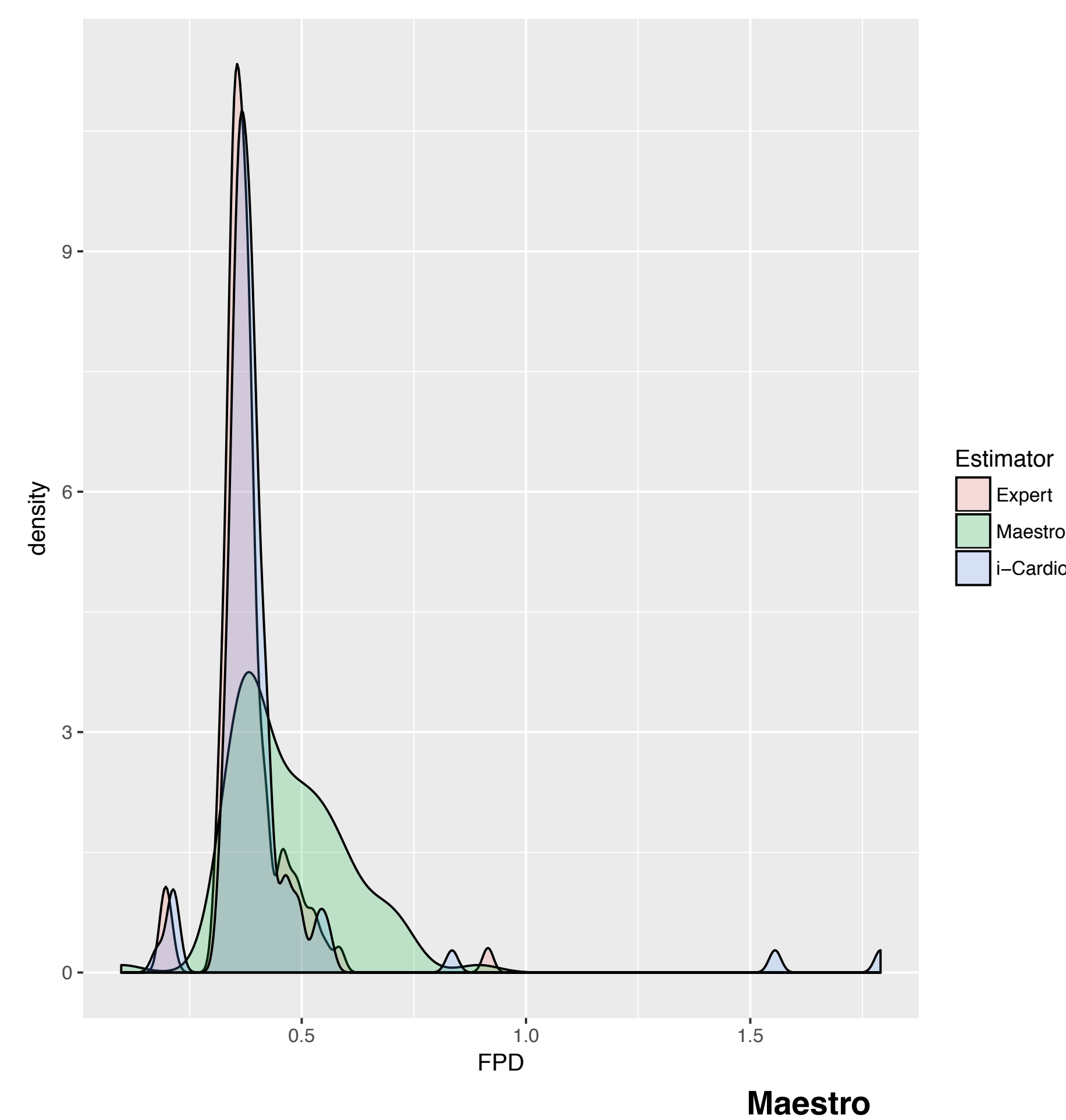
Fig.2: Distribution of FPD values estimated by three different methods: expert responses, the Maestro algorithm and the i-Cardio algorithm. We observe a strong similarity between the i-Cardio results and the expert's values.
