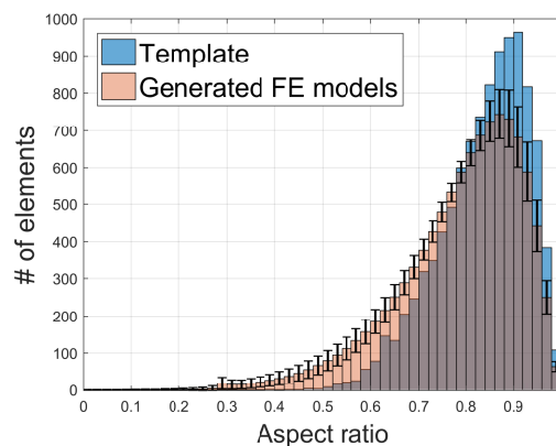
(b) Histogram of the mean AR over 1000 randomly generated shapes. The errorbar corresponds to one standard deviation. The template AR histogram is also represented to provide a ground truth.
