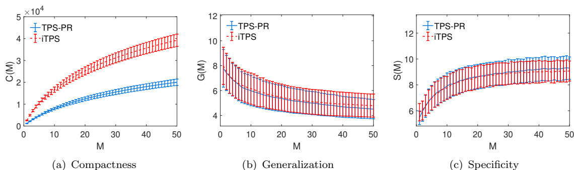
Figure 3. Comparison of the methods for the liver database (compactness, generalization and specificity). For a given number of modes lower values mean a better method. The error bar is one standard deviation.
