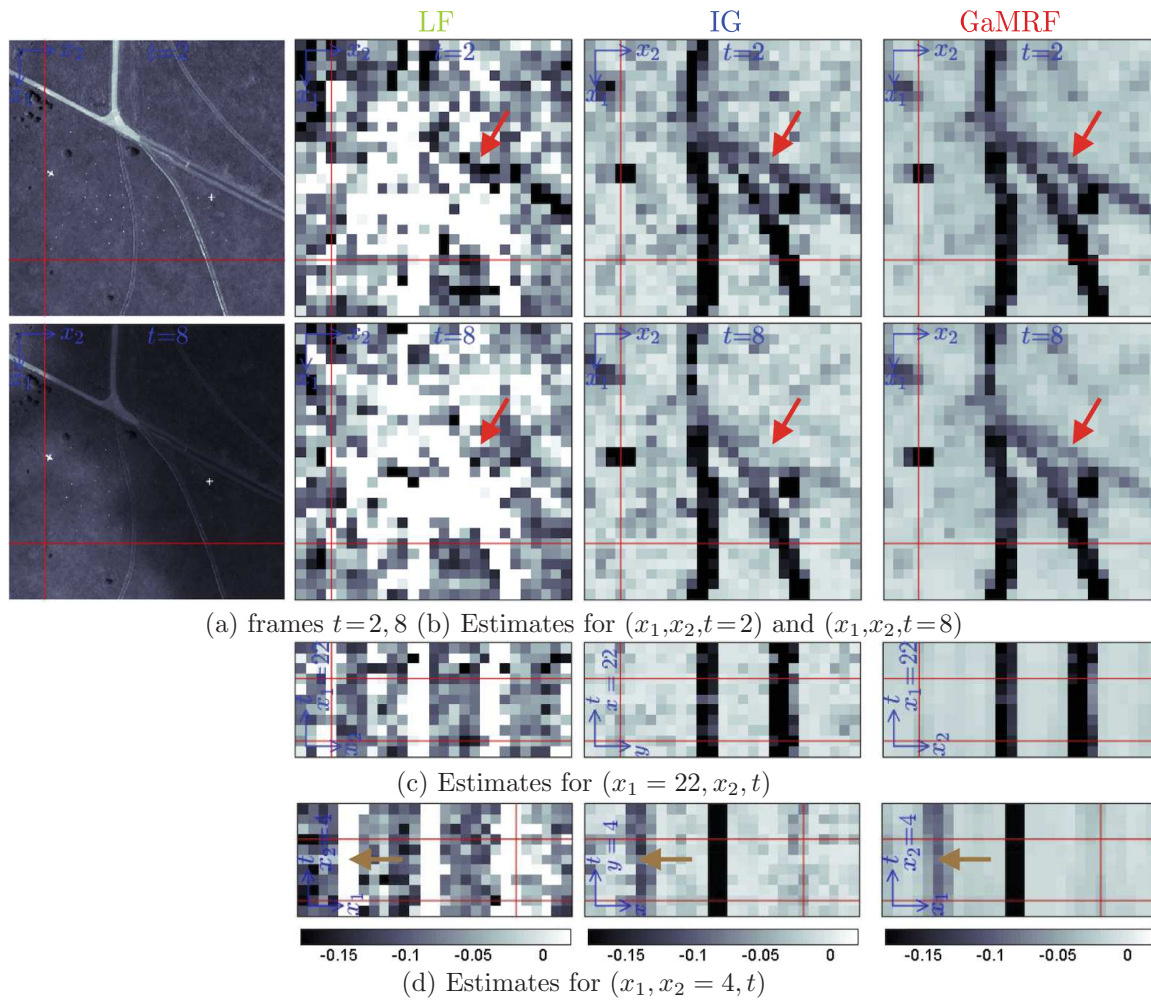
Figure 5. Multifractal analysis of a multitemporal image.
