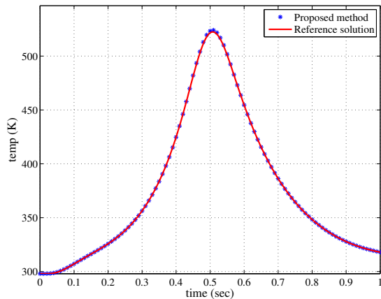
Figure 6: Single-ply composite cylinder: comparison of the temperature evolution at point \boldsymbol{x}_0 for a moving heat flux on the outer boundary for the proposed PGD-based solution (discontinuous blue) and the standard FE (solid red).
