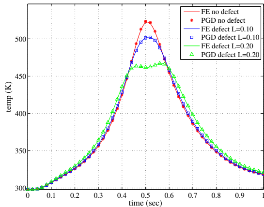
Figure 9: Multi-ply composite cylinder: comparison of the temperature evolution at point \mathbf{x}_0 for the proposed PGD-based solution (discontinuous) and the standard FE (solid) for different defect lengths.
