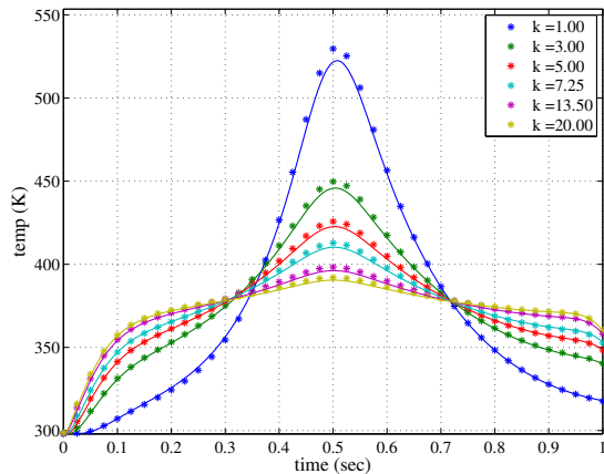
Figure 13: Multi-parametric comparison of the temperature evolution at point \boldsymbol{x}_0 for the proposed PGD-based solution (discontinuous) and the standard FE (solid) for thermal conductivities.
