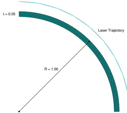
Figure 1: Single-ply composite cylinder: problem statement.
