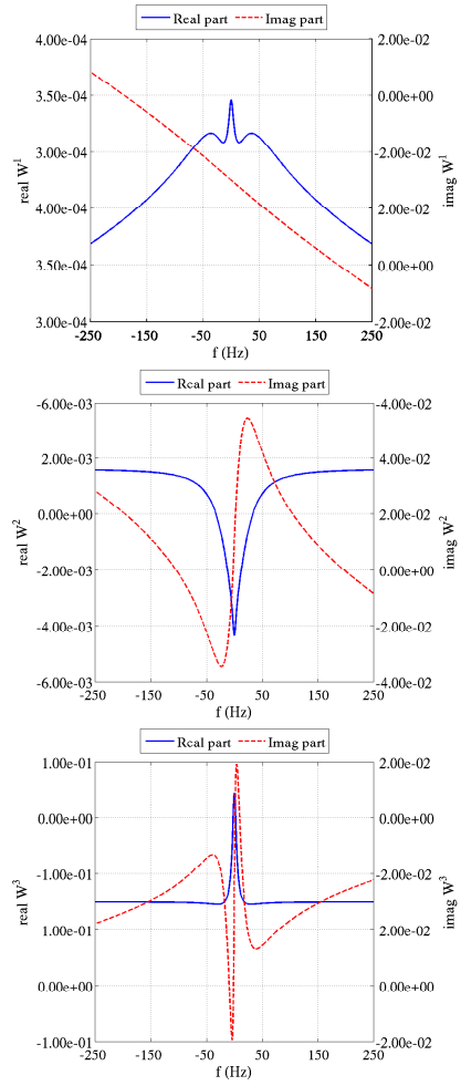
Figure 4: Single-ply composite cylinder: first 3 PGD frequency modes.
