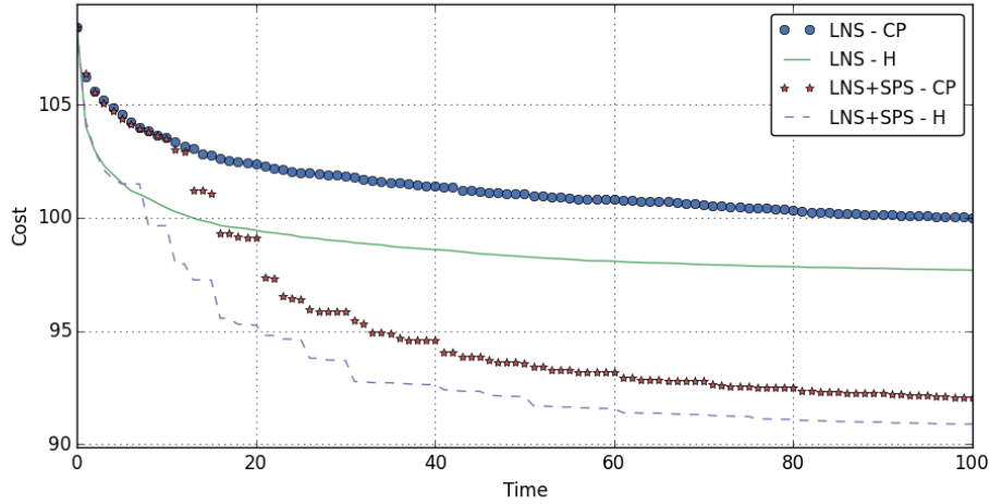
Figure 3: Comparison of the evolution of the average solution quality over time (in percentage of time limit) for four different configurations: with CP solver/with heuristics tests, with/without SPS. The results aggregate 5 runs for each dock value in the shared case for instances in the training set. They have been normalized, first by instance then by method, with 100 representing the cost at the end of LNS with CP solver tests (LNS-CP)
