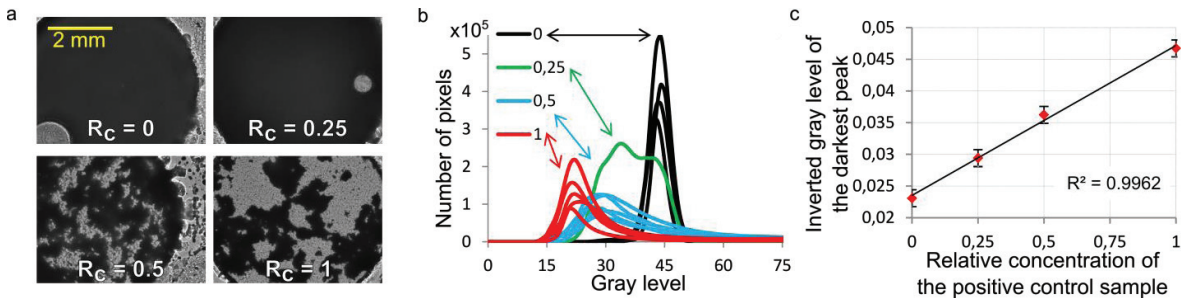
Fig. 1. a) Lens-free images of the 150 \mu\text{m} thick microfluidic chambers, b) gray levels histograms and c) inverse of the darkest peak gray level for various concentrations of D-dimers.
