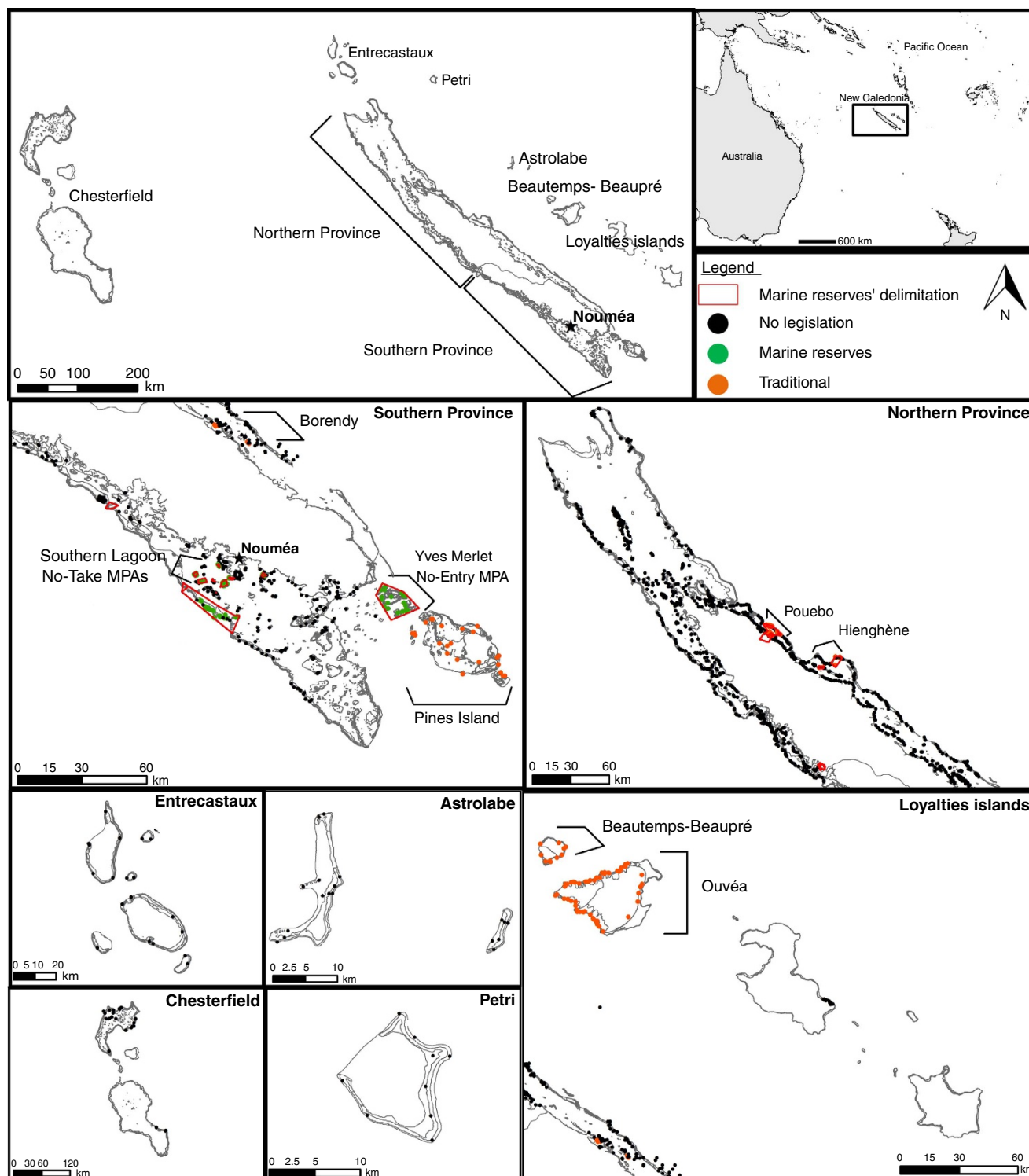
Figure 1 | Location of study areas in New Caledonia. Sites were located at the outer reef, back reef, lagoon reef or fringing reef depending on the locations and configurations of the reefs. Reef fishes and habitats were surveyed at each transect. Transects (1833) were performed between 1986 and 2013 in areas without legislation (black dots), in marine reserves (green dots) and in traditionally managed areas (orange dots).
