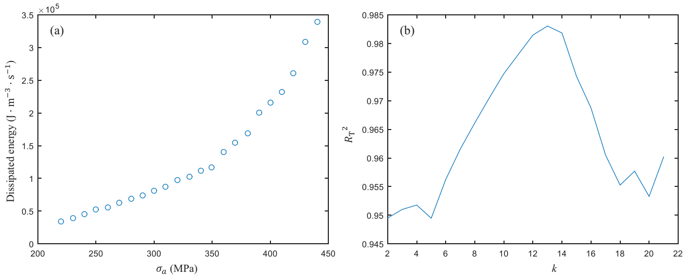
Fig. 9. Goodness of fit versus the sequence number of separated point. (a) Original experimental data from [31]. (b) Curve of R_r^2 versus split point number k .
