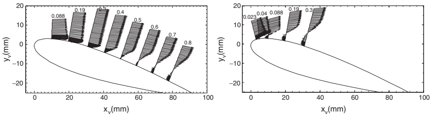
Fig. 10a Velocity profile for NACA0015 at 16^\circ corresponding to state I ( left ) and state II ( right )
