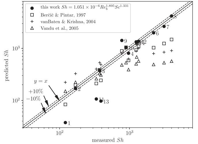
Fig. 17. Comparison of Eq. (15) to available scaling laws from literature.
