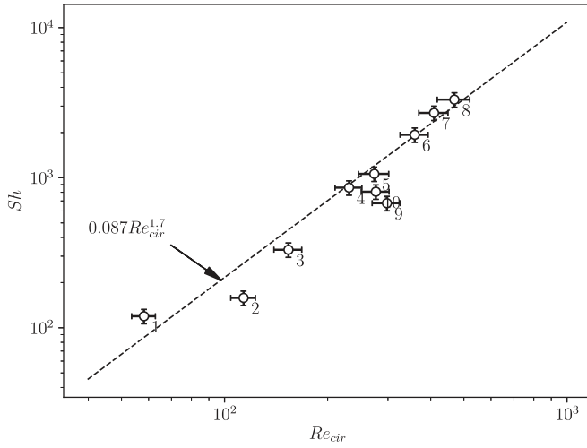
Fig. 16. Re_{cir} vs Sh for all water regimes at Sc = 526 .
