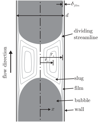
Fig. 10. Sketch showing the different characteristic dimensions and areas in the unit cell.
