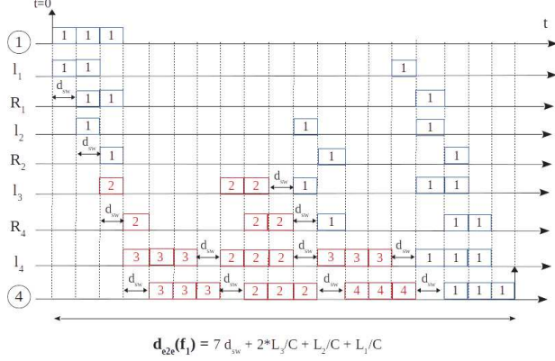
Figure 4: Case study 1: recursive calculus application for flow f_1 with Tiler NoC
