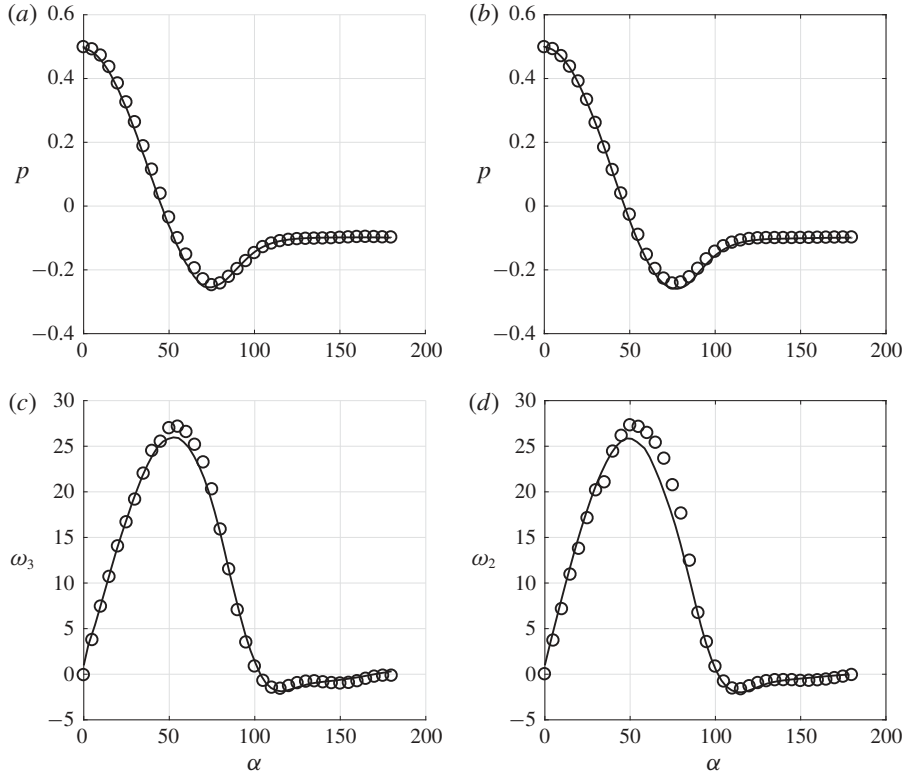
FIGURE 12. Surface pressure and non-zero components of the surface vorticity within the aa ( a,c ) and bb ( b,d ) cross-sectional planes for Re^{out} = 10^3 . Circles: DNS; solid line: macroscopic result based on (2.28).
