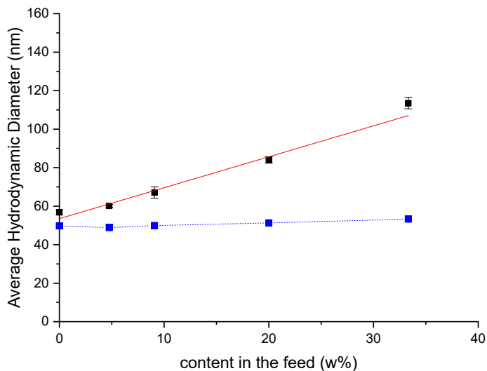
Figure 6. Average hydrodynamic diameter of mPEG 5K -b-p(HPMA-Bz) 18.5K in black/red as a function of homopolymer content in the feed, and in blue as a function of free mPEG 5K content in the feed (n=3).
