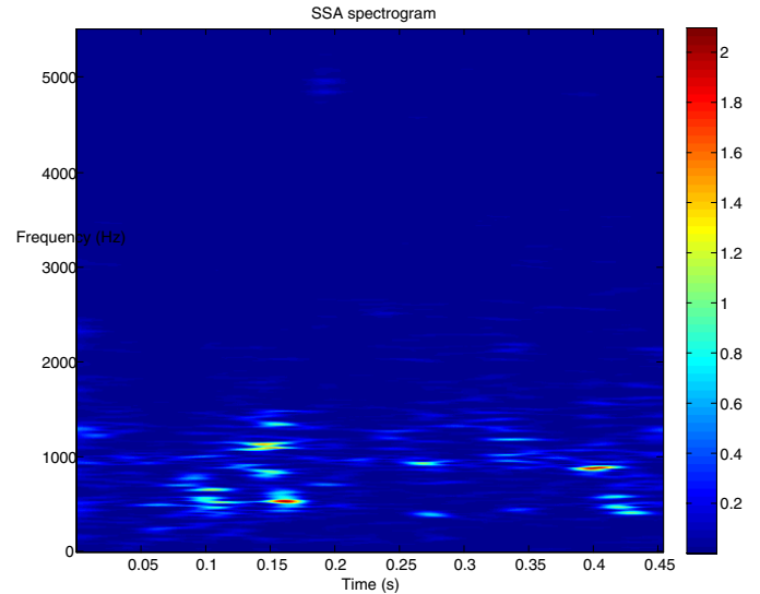
Fig. 3. Spectrogram (partial view, linear scale) of a shad spawning act (SSA). Right hand scale for signal power ( Volt^2 ).
