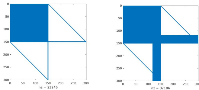
Figure 3 – Bad n \times n matrices for Karp-Sipser with t = 2 (left) and t = 32 (right).
