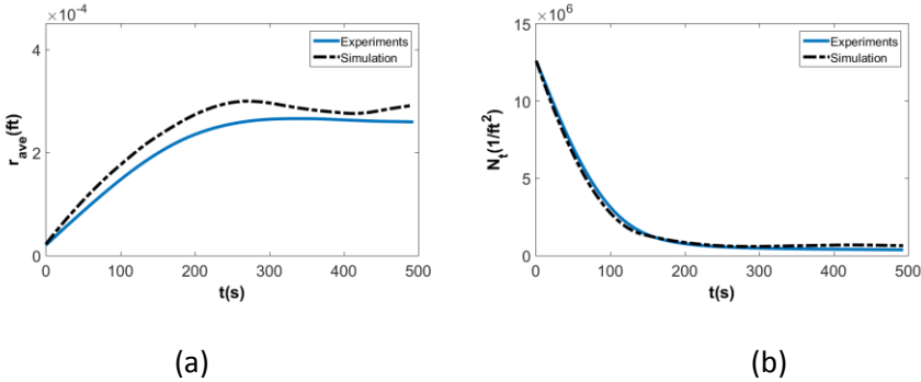
Figure1 Changes in (a)droplet size and (b) Nucleation site density for simulation and experiments
