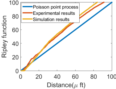
Figure2 Ripley function of progress at steady state
