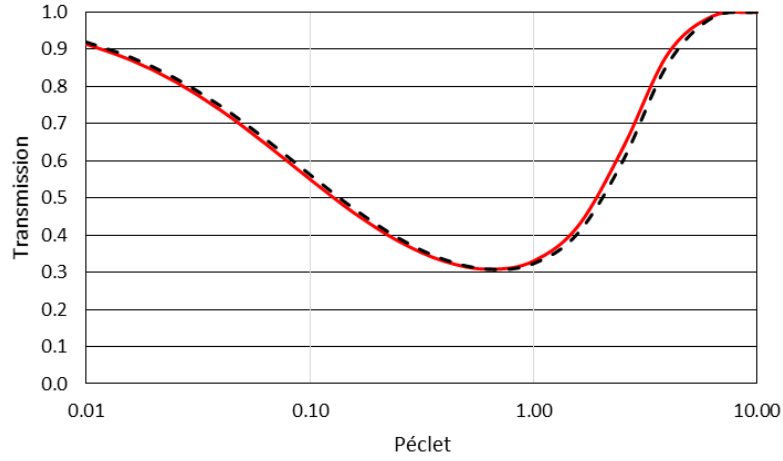
Figure 3. Modeling of the transmission during a filtration for different Peclet number, Pe = Pe_{MB} = Pe_{PL} . The model (full red line) is compared to the classical transmission model of Opong and Zydney [40].
