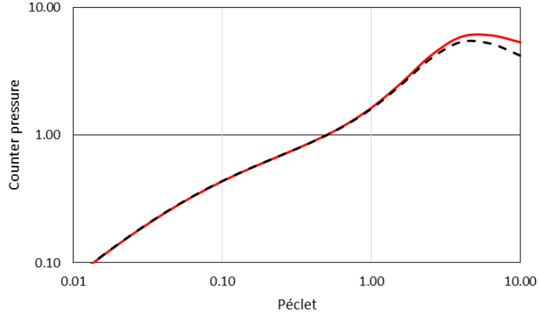
Figure 4. Modeling of the counter-pressure during a filtration for different Peclet number, Pe = Pe_{MB} = Pe_{PL} . The model (full red line) is compared to the Kedem Katchalsky approach (dashed line) with a Staverman coefficient, \sigma = (1 - K) .
