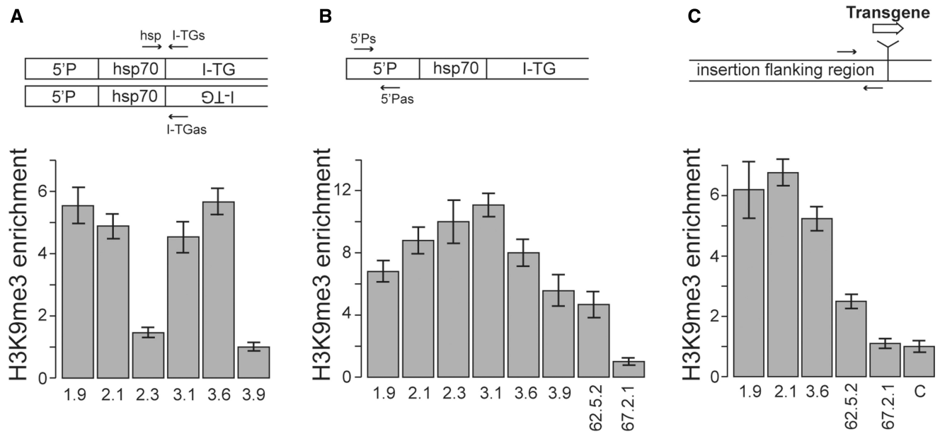
Figure 5. Chromatin status of the transgene-associated piRNA producing loci. ChIP was done using antibody specific to H3K9me3. (A) The ratio of normalized quantities of precipitated transgenic construct regions in I -transgenic strains to that in I -transgenic strain 3.9 (this strain produces the lowest amount of small RNAs mapping to the transgene). Locations of primers that amplify hsp70-I-TG transgenic regions in I -sense and I -antisense constructs are indicated above the graphs. (B) The ratio of normalized quantities of precipitated 5'-P-element transgenic construct regions (primers are indicated above) in I -transgenic strains to that in the I -promoterless strain 67.2.1 (C) The ratio of normalized amounts of precipitated transgene flanking regions in transgenic strains 62.5.2, 67.2.1, 1.9, 2.1 and 3.6 to that in w K or in strains with different transgene insertion sites (designated as C, for control). Error bars indicate standard deviation of triplicate PCR measurements. Primers specific to the flanking genomic regions adjacent to the 5'-P fragment of transgenes were used in this analysis (shown above the graph). Primers to 1.9, 2.1 and 3.6 flanking regions are shown in Figure 4.
