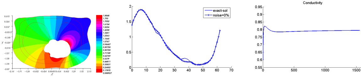
FIGURE 5. Reconstructed potential u_1 (left) and reconstructed Dirichlet condition (middle) compared to the exact solution on \Gamma_i for noise-free. The behaviour of the conductivity during iterations is also plotted (right). At convergence, the reconstructed conductivity k_3^{opt} = 0.794542 .
