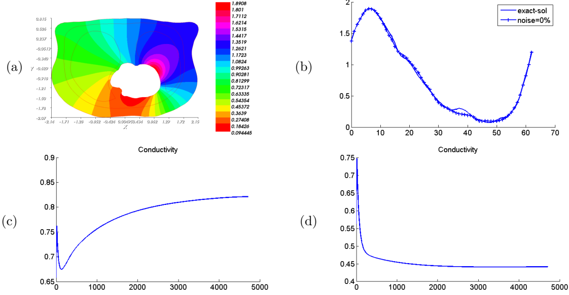
FIGURE 9. (a) Reconstructed potential u_1 in the domain, (b) reconstructed dirichlet condition on \Gamma_i . (c) The behaviour of the conductivities k_3 and (d) k_4 during iterations for noise free. At convergence, the conductivities are equal to k_3^{opt} = 0.821142 and k_4^{opt} = 0.441652 .
