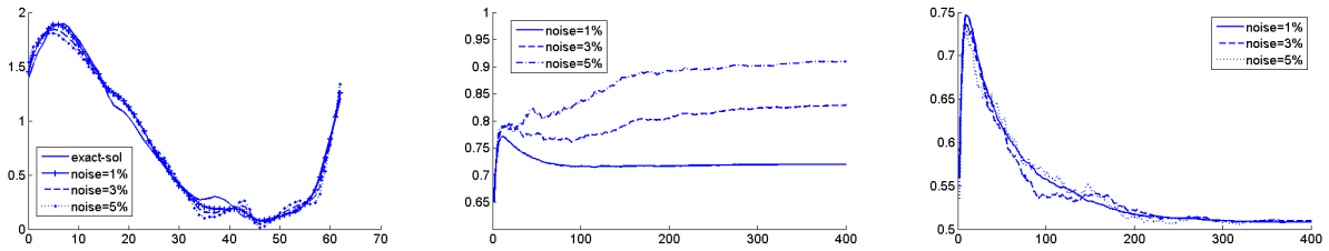
FIGURE 10. Reconstructed dirichlet condition on \Gamma_i (left) and the behaviour of the conductivities k_3 (middle) and k_4 (right) during iterations for different noise levels (1%, 3%, 5%).
