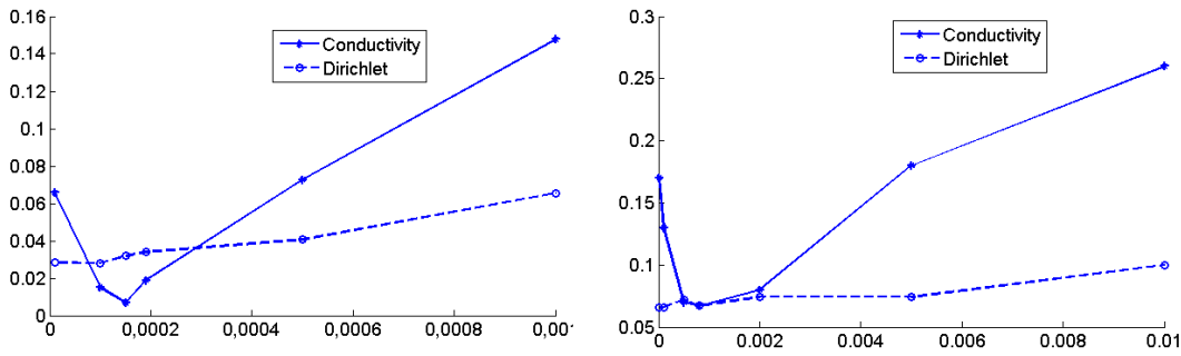
FIGURE 8. The conductivity error \frac{\|k^{ex} - k^{opt}\|_2}{\|k^{ex}\|_2} and Dirichlet error \frac{\|\tau^{opt} - u^{ex}\|_{\mathbb{L}^2(\Gamma_i)}}{\|u^{ex}\|_{\mathbb{L}^2(\Gamma_i)}} are presented with respect to different values of \alpha for noise free (left) and for 3% of noise (right).
