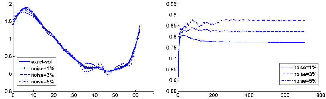
FIGURE 7. The reconstructed Dirichlet condition compared to the exact solution on \Gamma_i for different noise levels (1%, 3%, 5%) (left). The behavior of the conductivity during iterations of the optimization algorithm (right).
