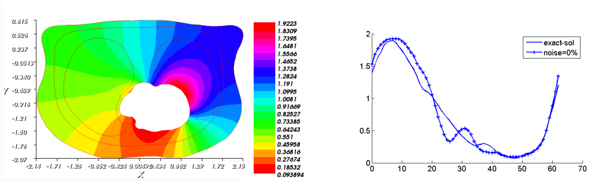
FIGURE 3. Reconstructed potential u_1 (left) and reconstructed Dirichlet condition (right) compared to the exact solution on \Gamma_i using an approximate value of k_3 = k_3^0 = 0.5 .
