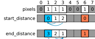
Fig. 2. Distance operators on a 8-bit bitmask. Only set pixels are considered.
