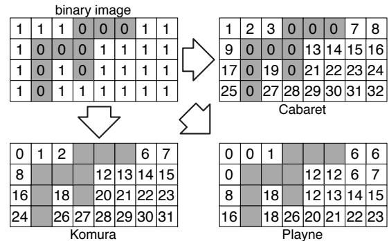
Fig. 1. Initialization on GPU for Cabaret, Komura and Playne algorithms
