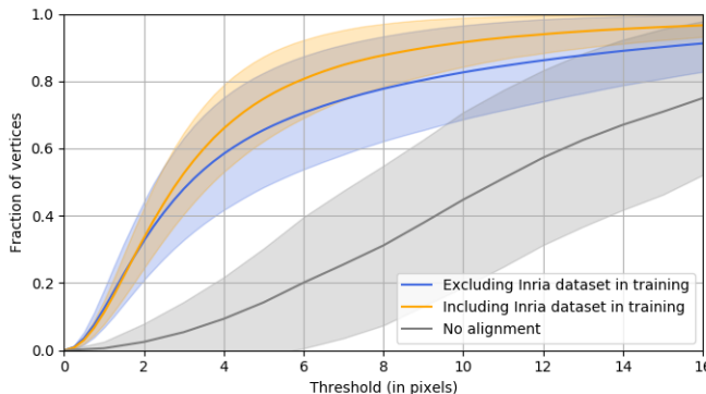
Fig. 1: Alignment accuracies. Solid curves are the average, shaded regions are within the standard deviation.
