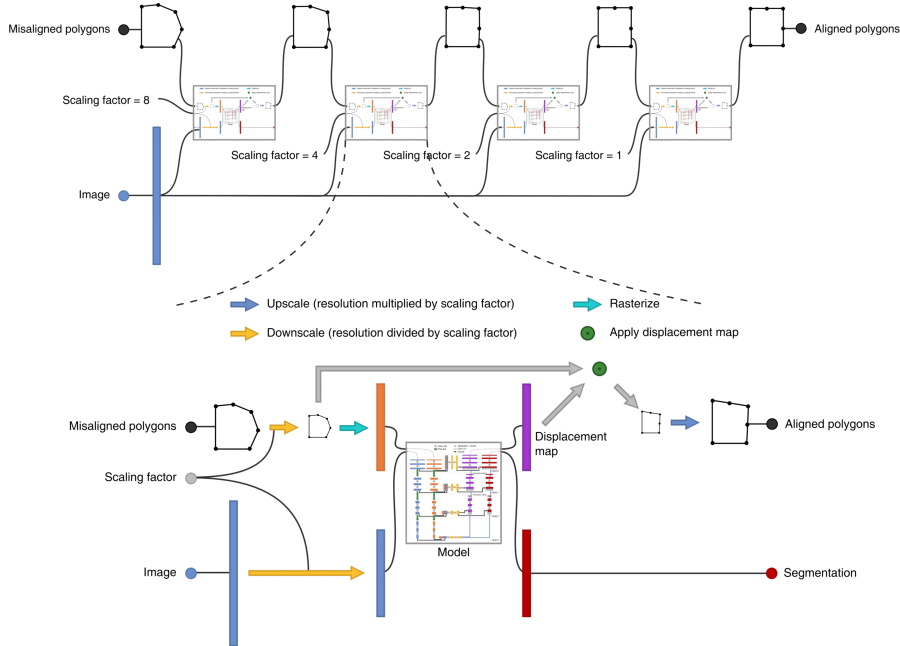
Fig. 4: Multi-resolution pipeline.
