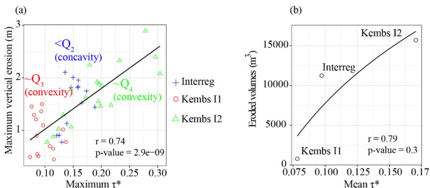
Fig. 3. Relations between (a) maximum vertical erosion and dimensionless peak flow shear stress calculated on each cross-section (flood intensity and gravel augmentation locations are indicated), and (b) eroded volumes and mean dimensionless peak flow shear stress for each artificial sediment deposit. Studied peak flows are those observed during the first flood events following the gravel augmentations (P1; see Fig. 2).
