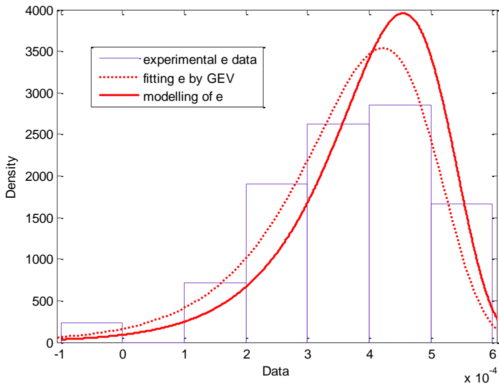
Figure 3. Distribution of error (e) fitted with EV and compared with model results (full line)
