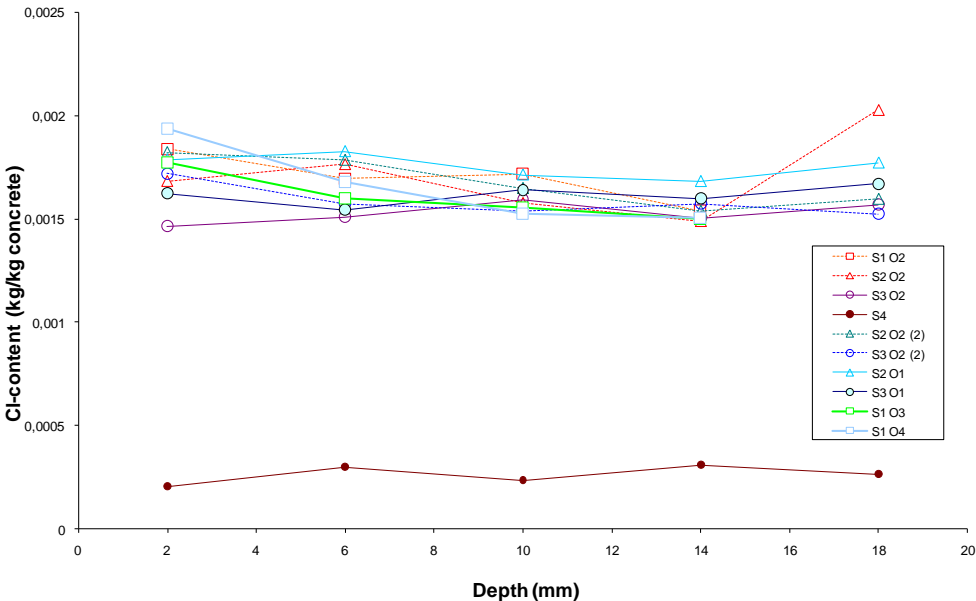
Figure 1. Total chloride profiles
