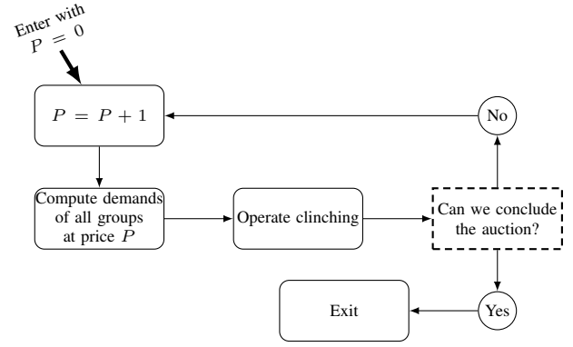
Fig. 2: Overview of the clinching approach for groups
