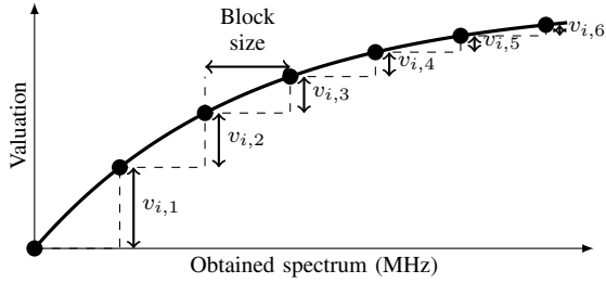
Fig. 1: An example of a concave valuation function of obtained spectrum, and the corresponding block valuations v_{i,n} for player i .
