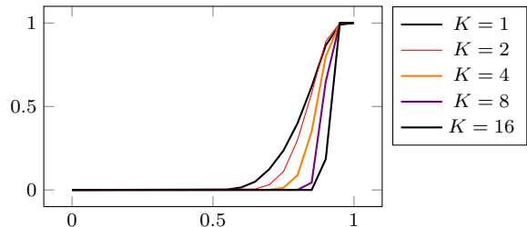
Fig. 6: Cumulative density function of SW_N as a function of the number of blocks for M = 10
