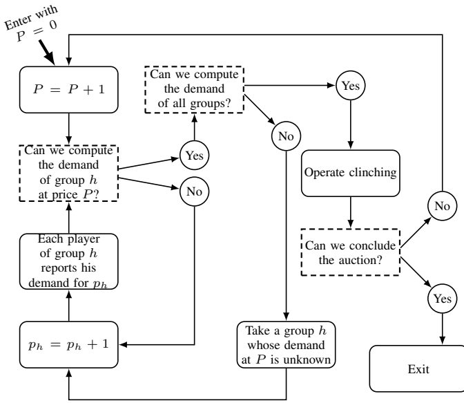
Fig. 4: C-LSA: applying the clinching approach in the LSA context
