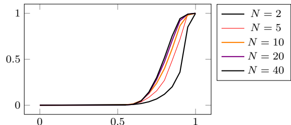
Fig. 7: Cumulative density function of SW_N as a function of the number of groups for K = 1
