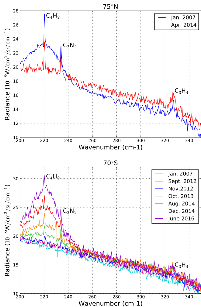
Fig. 8. Evolution of measured radiances at 75^\circ N (top panel) and 70^\circ S (bottom panel) from 2007 (northern winter) to 2016 (mid-spring). The sharp variation in the radiance between 228\text{ cm}^{-1} and 231\text{ cm}^{-1} in the spectra measured in August 2014 is a spurious noise feature which could not be eliminated during the calibration process. From 2007 to 2016, radiance at high southern latitudes has strongly increased, whereas it has decreased at high northern latitudes.
