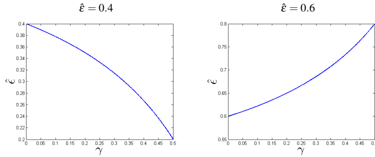
Fig. 1 Variations of the evidential error rate \hat{\varepsilon} with the uncertainty level \gamma when \tilde{\varepsilon} = 0.4 and 0.6
