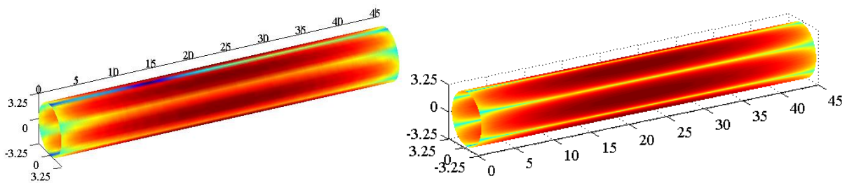
Figure 7: Radial acceleration (dB ref 1e-5 m/s 2 ) on the surface of the fluid-loaded cylindrical shell at the second resonance peak corresponding to 3.6 Hz using FEM/BEM (left) and 3.7 Hz using CTF (right).
