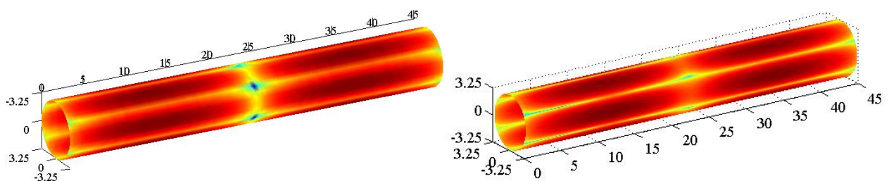
Figure 8: Radial acceleration (dB ref 1e-5 m/s 2 ) on the surface of the fluid-loaded cylindrical shell at the third resonance peak corresponding to 4.4 Hz using FEM/BEM (left) and 4.7 Hz using CTF (right).
