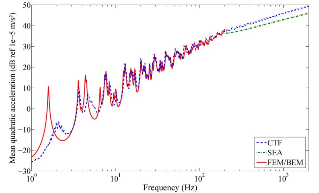
Figure 5: Mean quadratic acceleration of the fluid-loaded cylinder.
