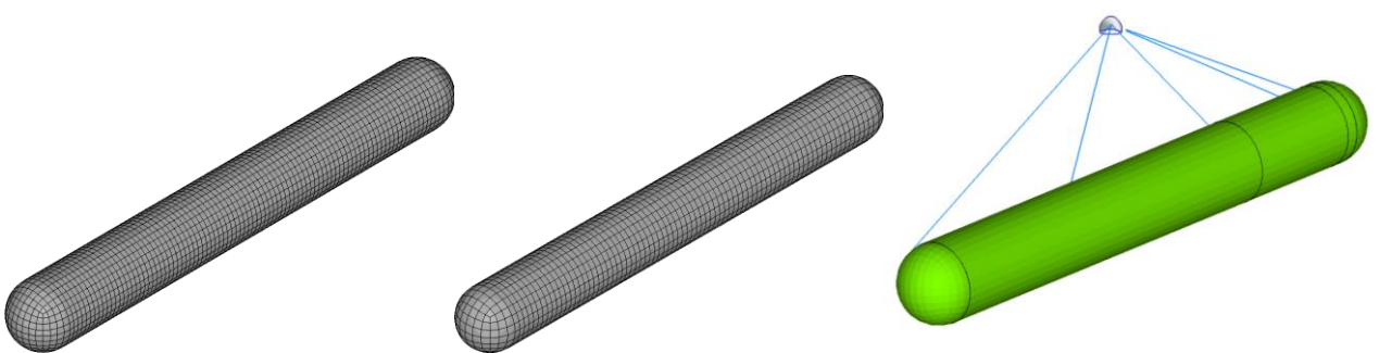
Figure 2: FEM mesh (left) and BEM mesh (right).
