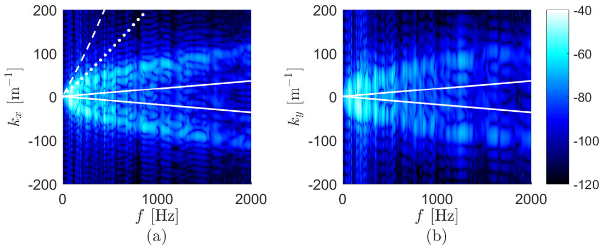
Figure 8: Squared absolute value of the sensitivity functions |H_v(\mathbf{x}, \mathbf{k}, f)|^2 (dB, ref. 1 \text{ m}^2 \cdot \text{s}^{-2} \cdot \text{Hz}^{-1} ) of panel B: (a) along k_x \geq 0 for k_y = 0 . (b) along k_y \geq 0 for k_x = 0 . The superimposed lines represent: k_0 (continuous line); k_c for U_\infty = 20 \text{ m} \cdot \text{s}^{-1} (dotted line); k_c for U_\infty = 40 \text{ m} \cdot \text{s}^{-1} (dashed line).
