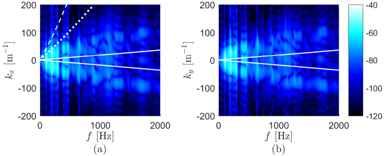
Figure 7: Squared absolute value of the sensitivity functions |H_v(\mathbf{x}, \mathbf{k}, f)|^2 (dB, ref. 1 \text{ m}^2 \cdot \text{s}^{-2} \cdot \text{Hz}^{-1} ) of panel A: (a) along k_x \geq 0 for k_y = 0 . (b) along k_y \geq 0 for k_x = 0 . The superimposed lines represent: k_0 (continuous line); k_c for U_\infty = 20 \text{ m} \cdot \text{s}^{-1} (dotted line); k_c for U_\infty = 40 \text{ m} \cdot \text{s}^{-1} (dashed line).
