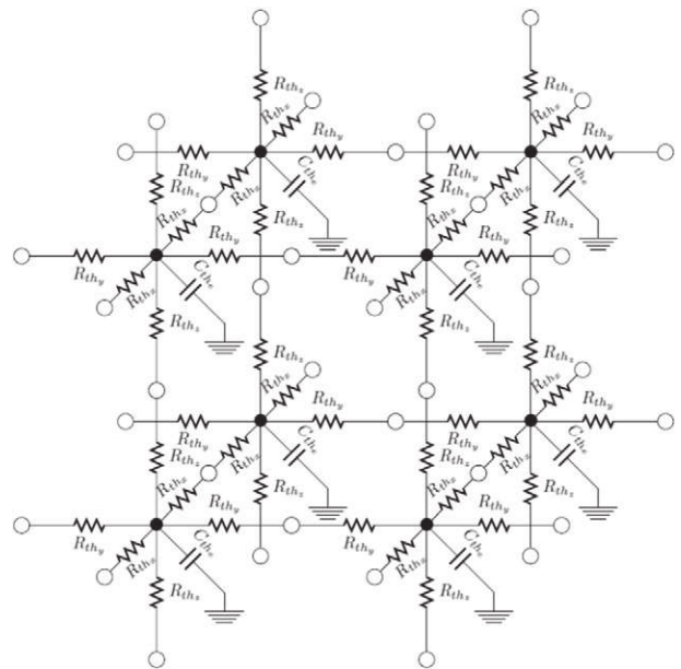
Fig. 2. Electrothermal nodal model of association of 8 elementary volumes.
