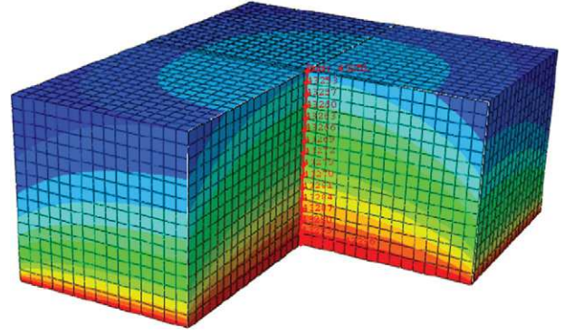
Fig. 7. Thermal field in silicone gel block.
