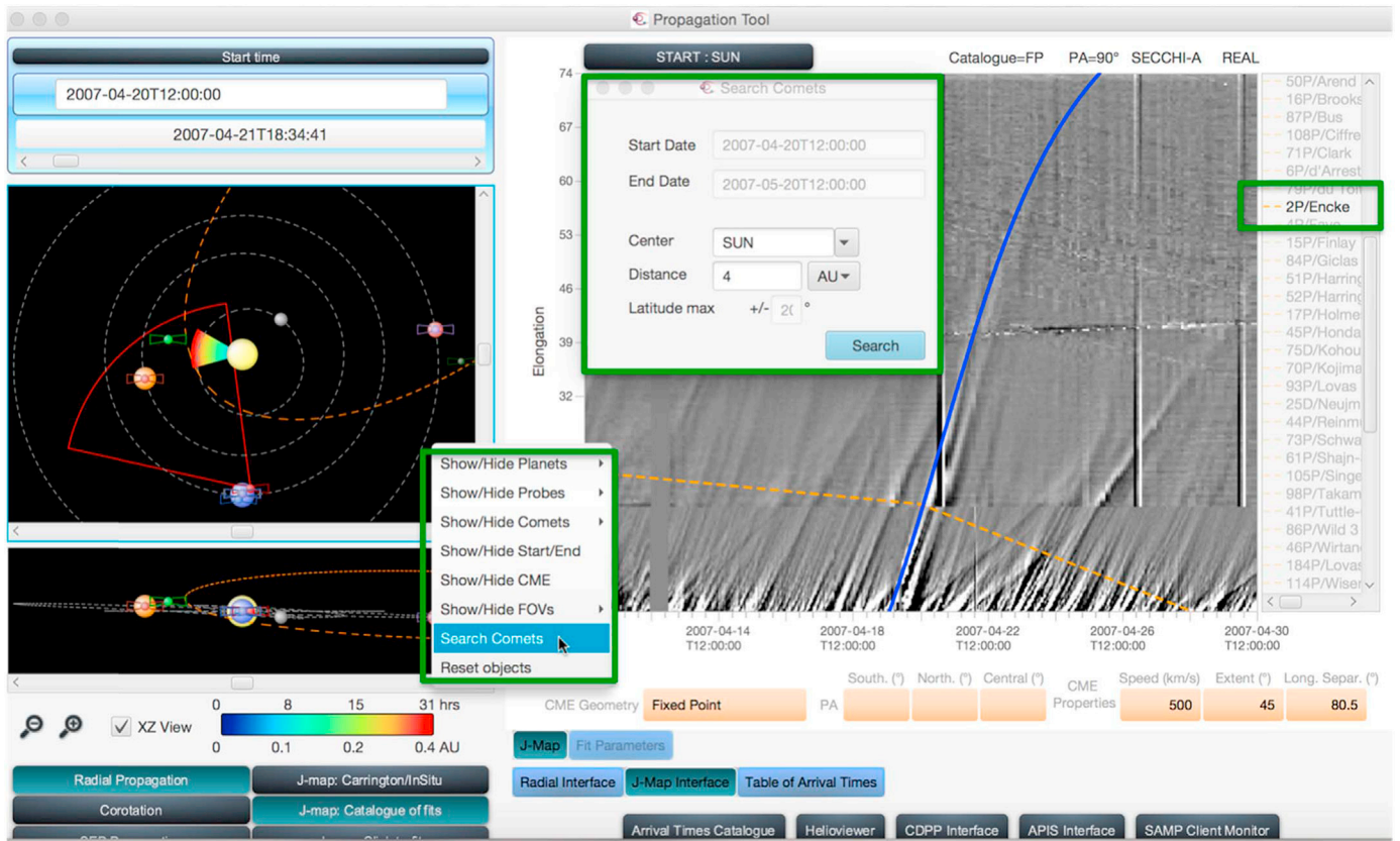
Fig. 5. Illustration of the new PSWS functionality implemented within the CDDP Propagation Tool and dedicated to comets. Green box: search window to identify comets flying by a central body at a particular distance during the selected time period. Once a comet is identified and selected (here 2 P/Encke), its orbit is displayed on the left in red-dashed line. Its location in a J-map obtained from STEREO-A observations is displayed on the right in orange-dashed line. The blue line corresponds to a particular CME identified from a catalogue of fits. (For interpretation of the references to color in this figure legend, the reader is referred to the web version of this article).
