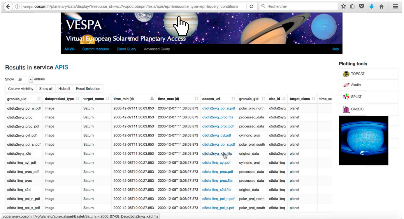
Fig. 3. Results of an EPN-TAP query from the VESPA interface searching for Saturn observations during the time period 01/11/2000-15/12/2000 in the APIS service.
